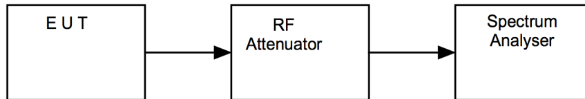
Figure vii Test Setup
