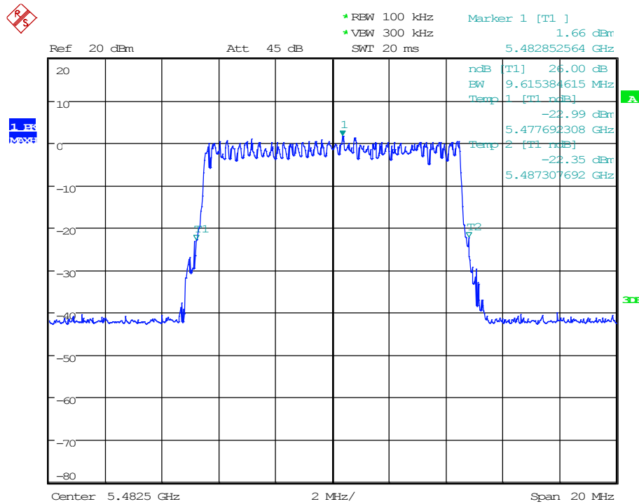
Channel 0 : 5482.5 MHz : 26 dB bandwidth
