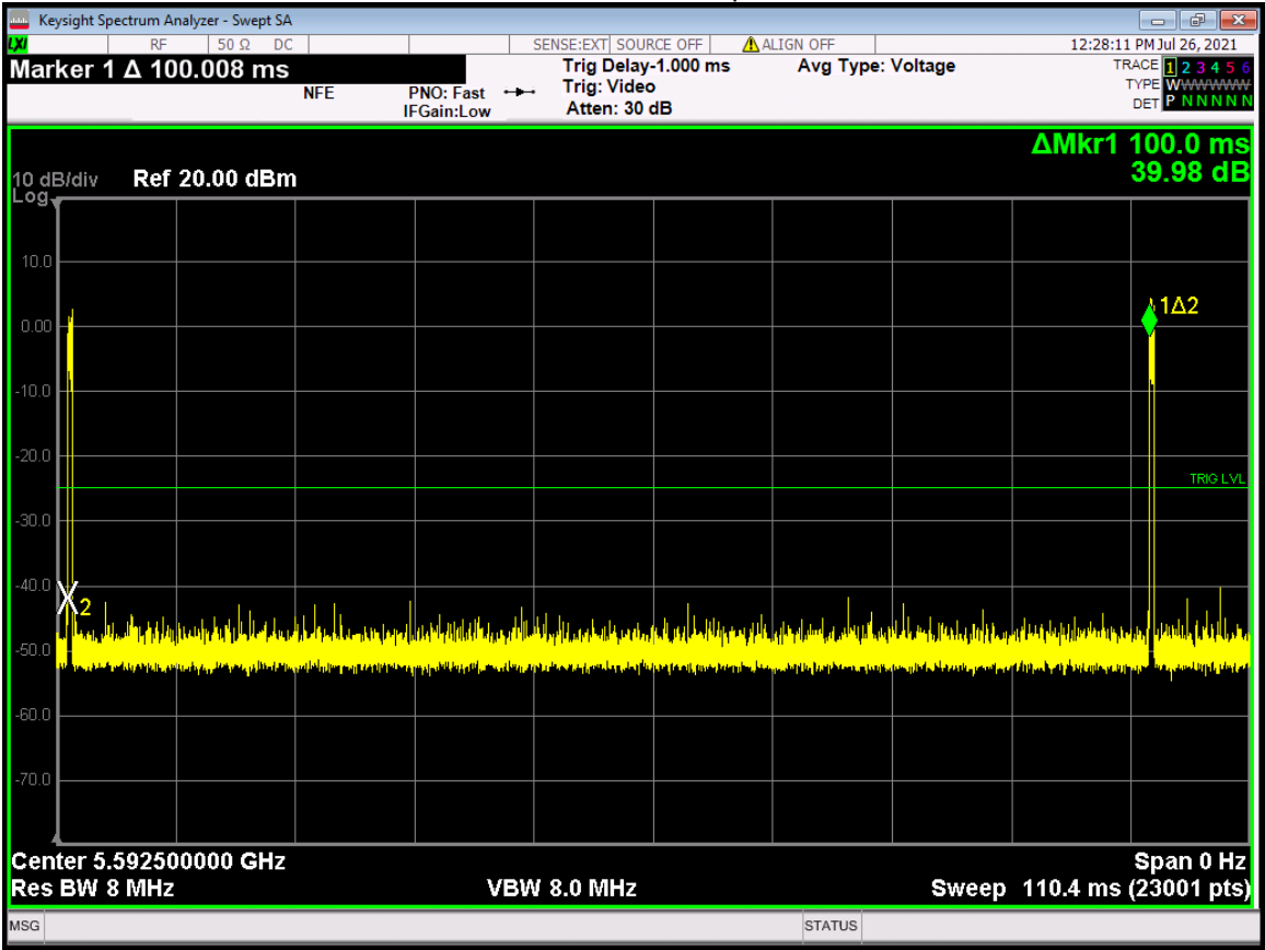
Channel 11 : 5592.5 MHz : Repetition interval
