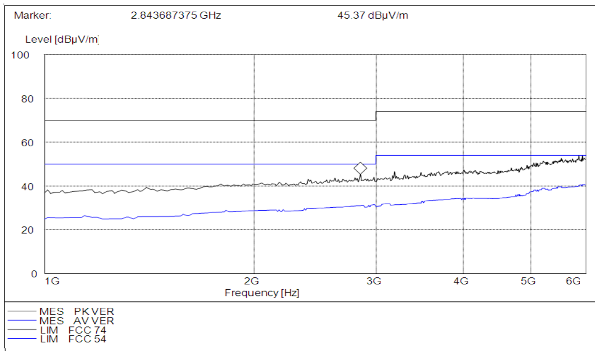
(Plot H: Test Antenna Vertical 1G – 6G)
