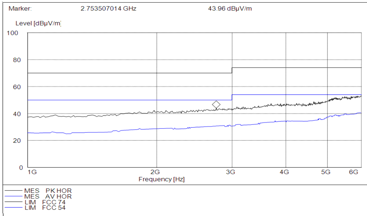
(Plot G: Test Antenna Horizontal 1G – 6G)
