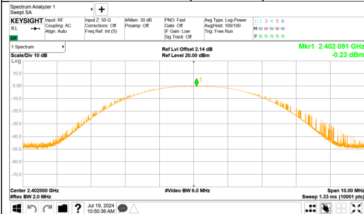
Channel 0 (2402MHz)
