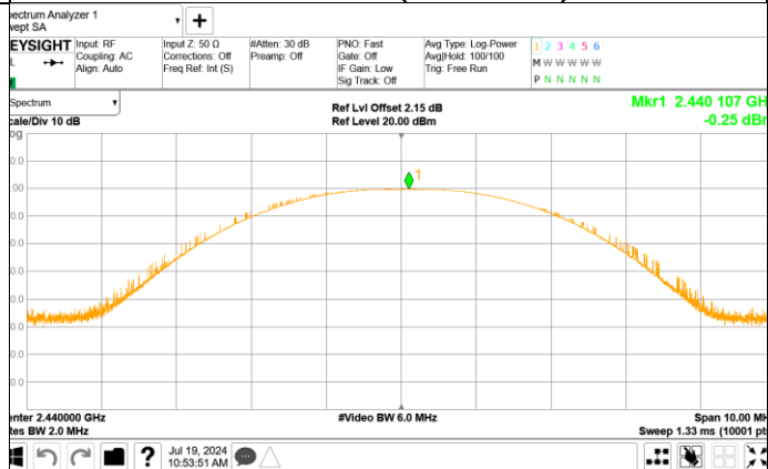
Channel 19 (2440MHz)
