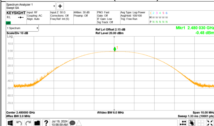
Channel 39 (2480MHz)
