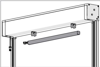
Screws need to be installed from inside Cassette to avoid fabric.
