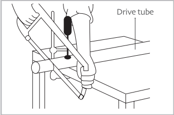
Cut roller tube to required length & de-burr.
