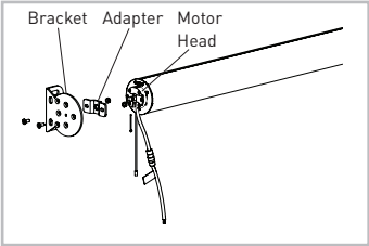
Mount motorized tube onto brackets.
