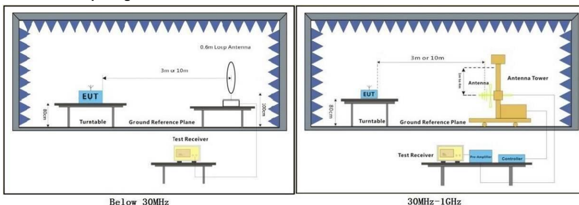
Below 30MHz
