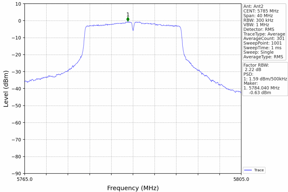
802.11ac(VHT20)_MCH_5785MHz_MIMO_NTNV
