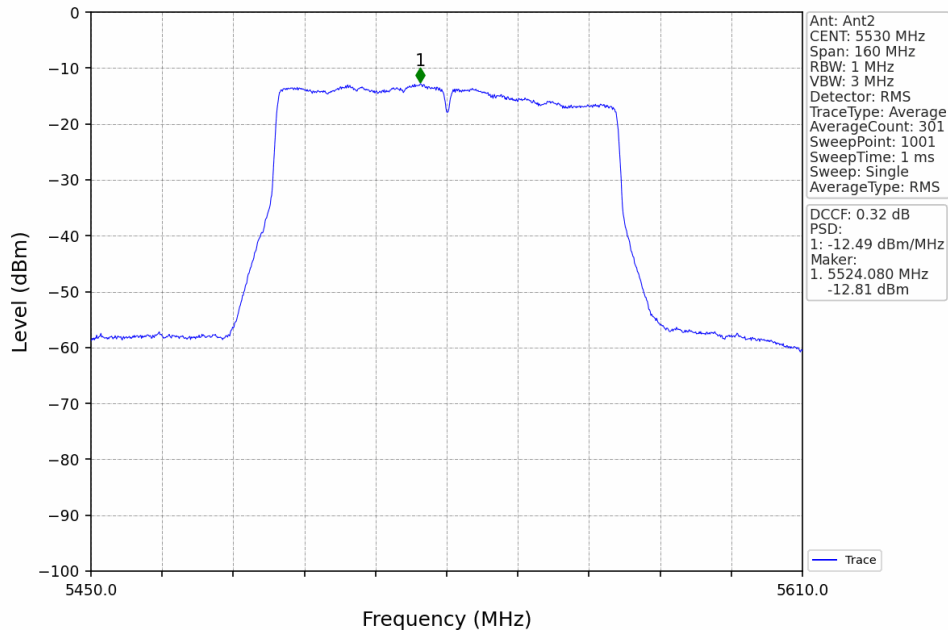
802.11ac(VHT80)_LCH_5530MHz_MIMO_NTNV
