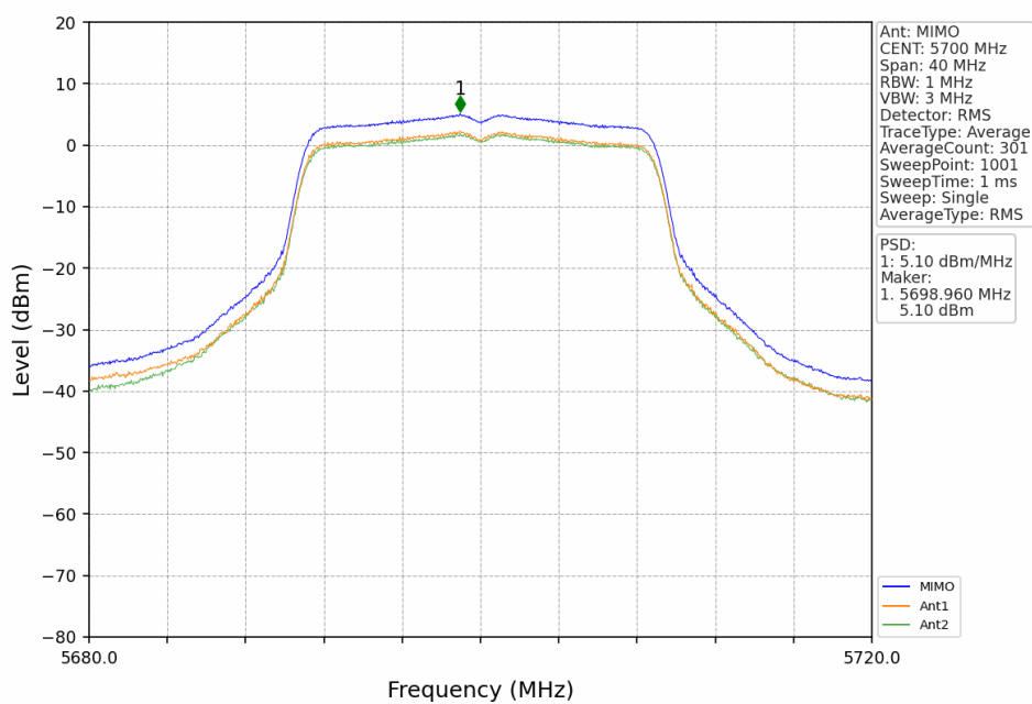
802.11ac(VHT20)_HCH_5700MHz_MIMO_NTNV
