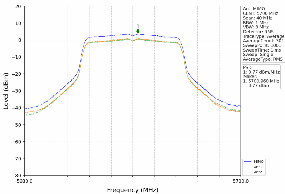
802.11n(HT20)_HCH_5700MHz_MIMO_NTNV
