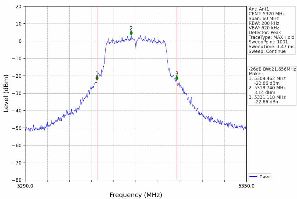
802.11a_HCH_5320MHz_Ant1_NTNV
