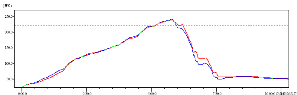
Figure 10. Reflow Soldering Profile
