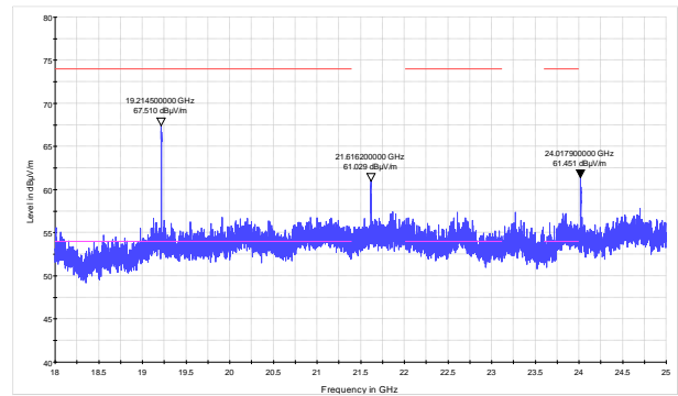
Figure 8.7-15: Radiated spurious emissions above 18 GHz, low channel
