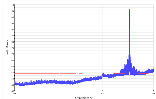
Figure 8.7-11: Radiated spurious emissions within 1–3 GHz, high channel
