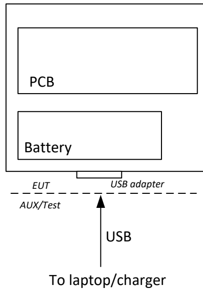
Figure 3.6-1: Setup diagram
