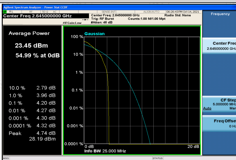
Band41-20MHz-QPSK-41140-100RB#0
