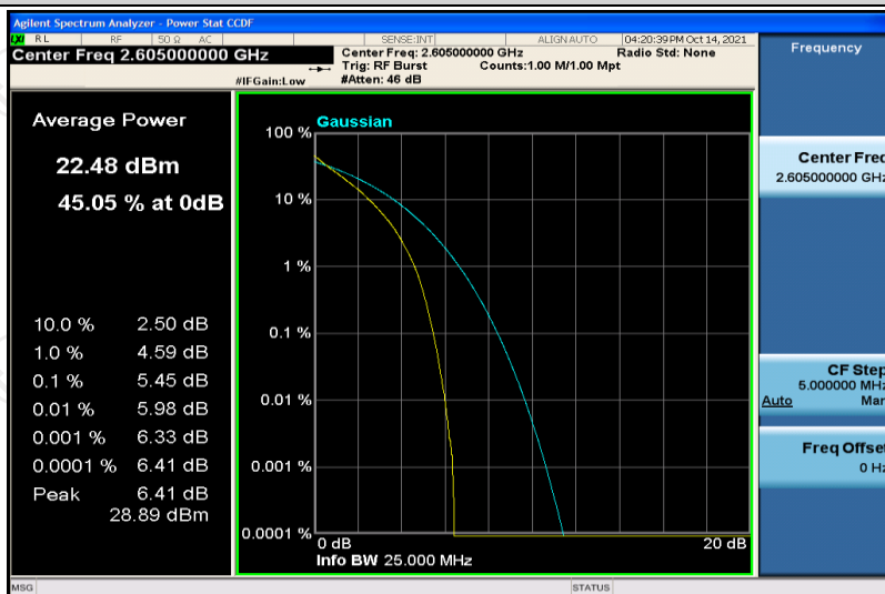
Band41-10MHz-QPSK-41190-1RB#0
