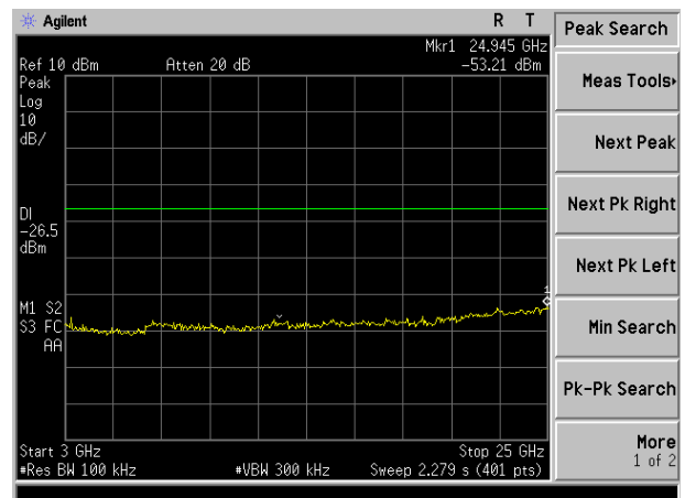
High Channel 2462MHz
