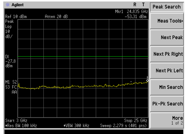
Middle Channel 2437MHz
