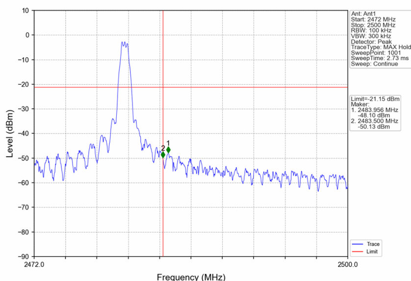
1M_HCH_2480MHz_Ant1_NTNV
