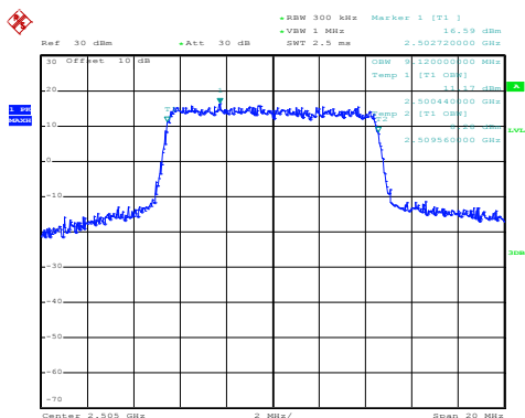
Modulation: 16OAM
