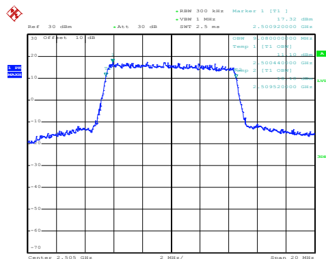
Modulation: OPSK
