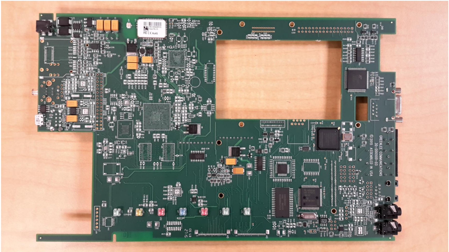
Figure 1 - PCB Side 1
