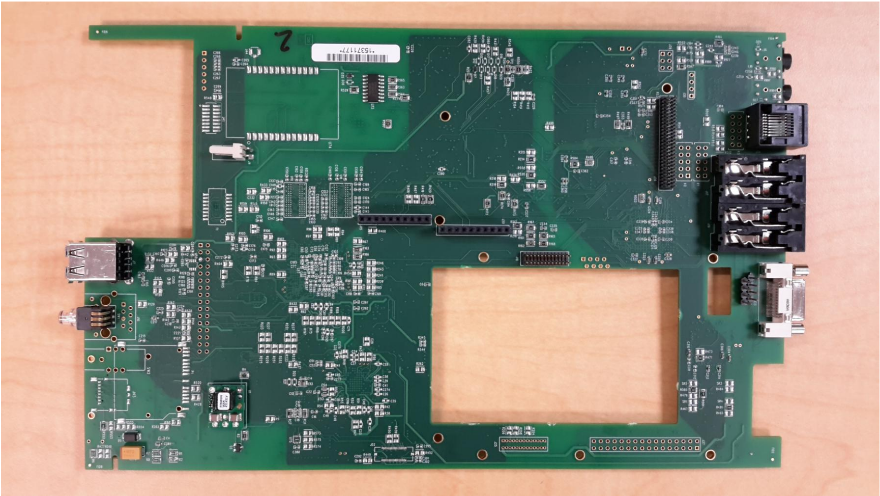
Figure 2 - PCB Side 2
