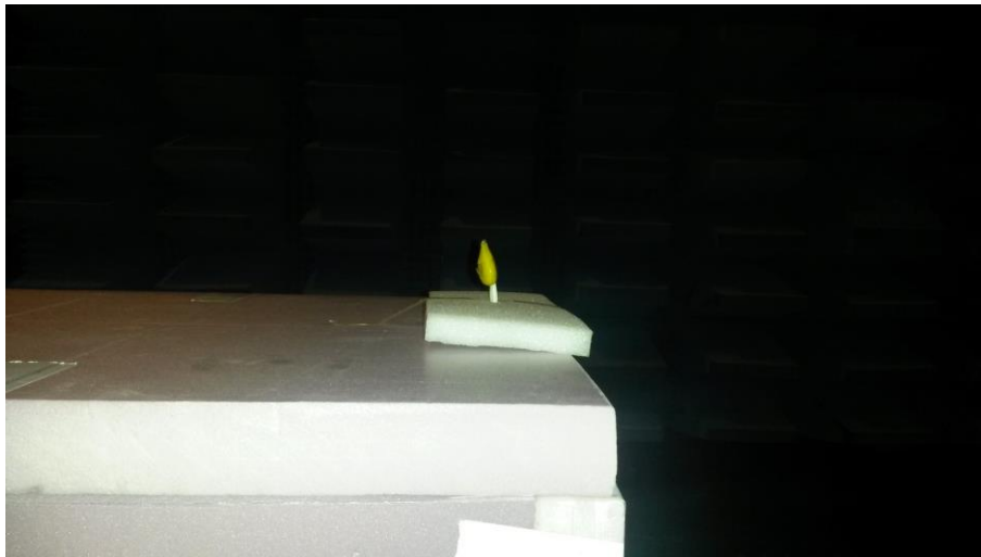
Radiated Emissions Setup in Semi-Anechoic Chamber, Above 1GHz
