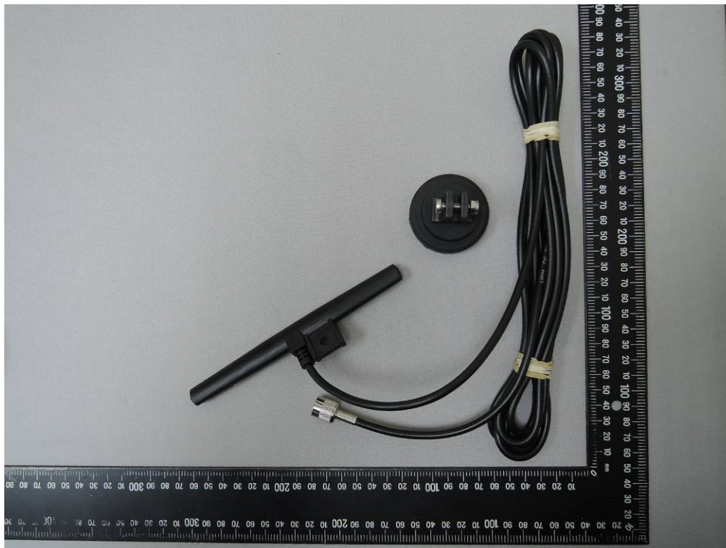
WWAN Antenna-4 (Model No.: FINDIPMAG, Supplier: Carant)
