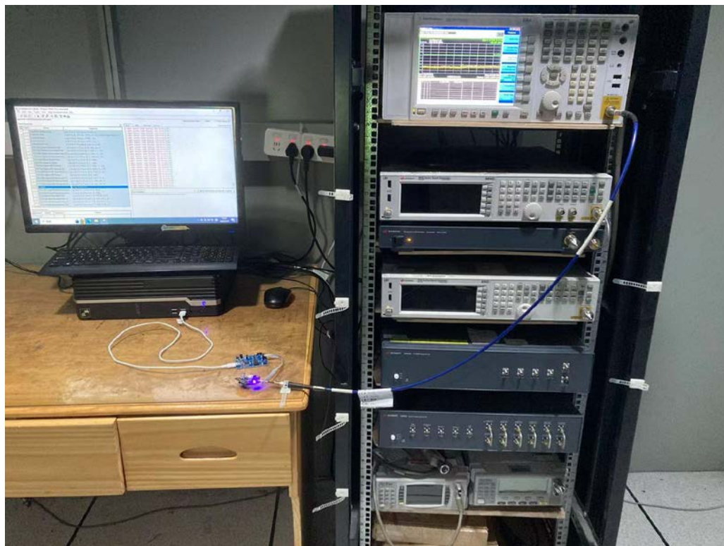
ANTENNA-PORT CONDUCTED
