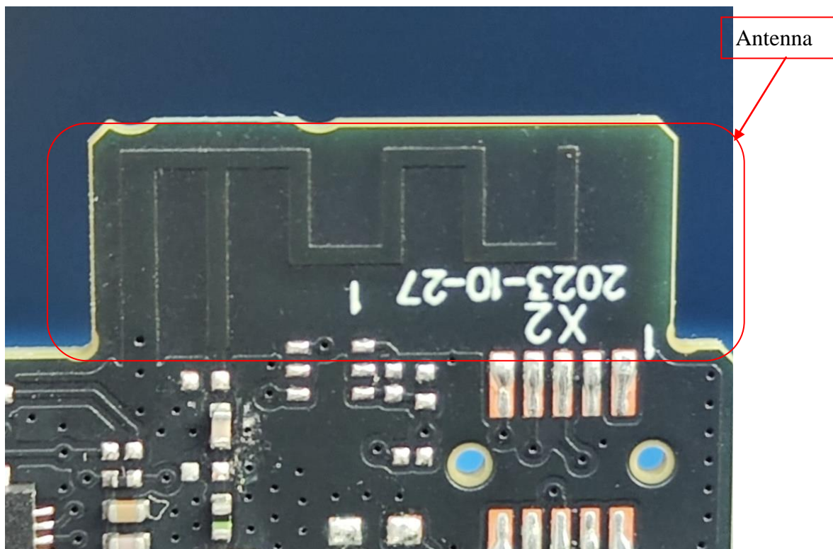
FIGURE 11 SENSOR (SC100B/02 SR TRANSCEIVER WH) ANTENNA
