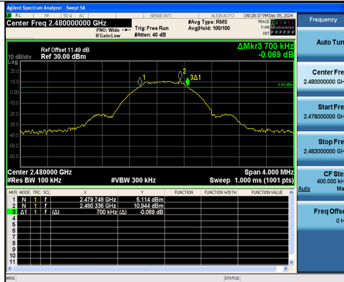
BLE_1M-Ant1-2480-PASS
