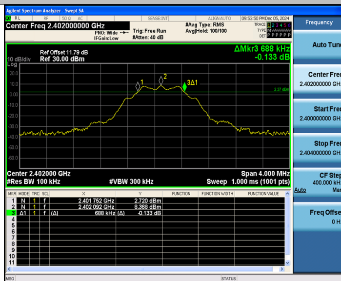
BLE_125K-Ant1-2402-PASS
