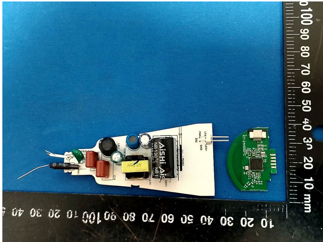
BLE&ZigBee Antenna
