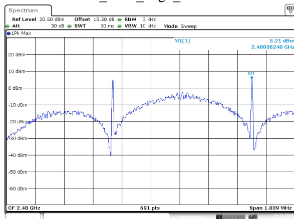
BLE_125k_High_Channel
