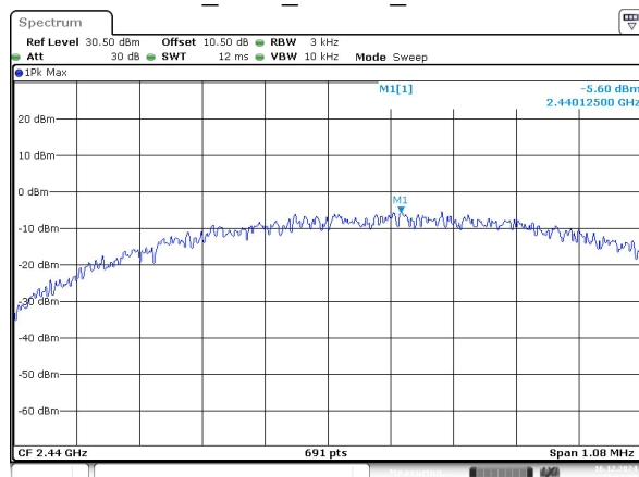
BLE_500k_Middle_Channel
