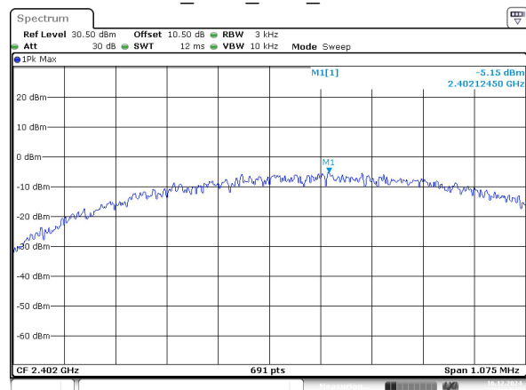
BLE_500k_Low_Channel
