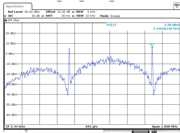
BLE_125k_Middle_Channel
