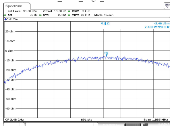
BLE_500k_High_Channel
