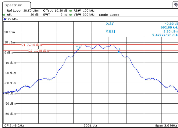
BLE_125k_High_Channel
