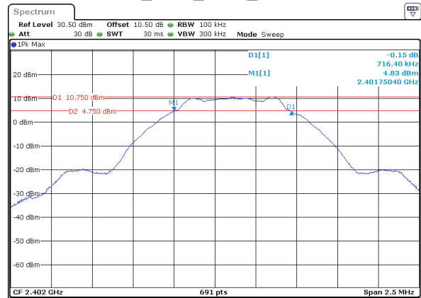
BLE_500k_Low_Channel
