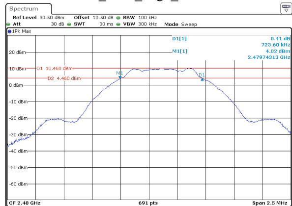
BLE_500k_High_Channel
