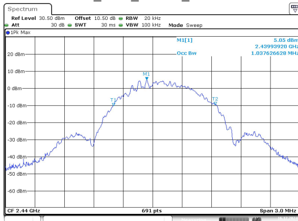
BLE_500k_Middle_Channel
