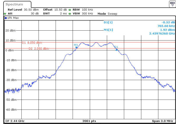
BLE_125k_Middle_Channel
