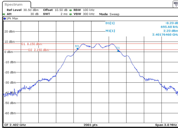
BLE_125k_Low_Channel
