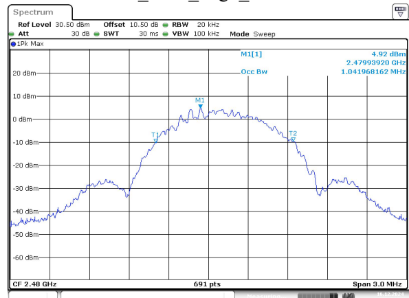
BLE_500k_High_Channel
