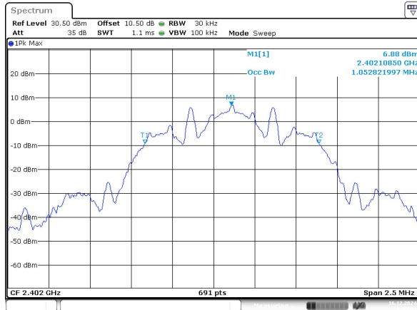
BLE_125k_Low_Channel
