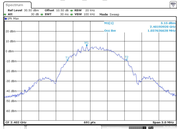
BLE_500k_Low_Channel
