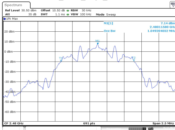
BLE_125k_High_Channel
