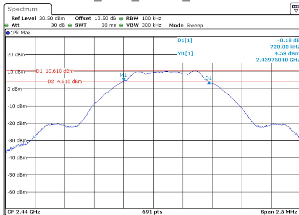
BLE_500k_Middle_Channel
