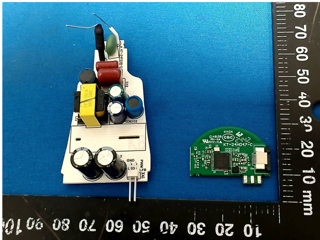
BLE&ZigBee Antenna
