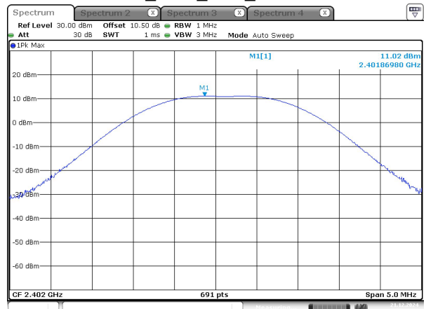
BLE_500k_Low_Channel
