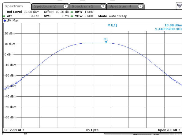
BLE_500k_Middle_Channel
