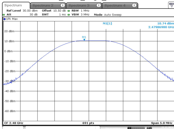
BLE_125k_High_Channel
