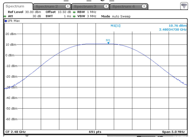
BLE_500k_High_Channel
