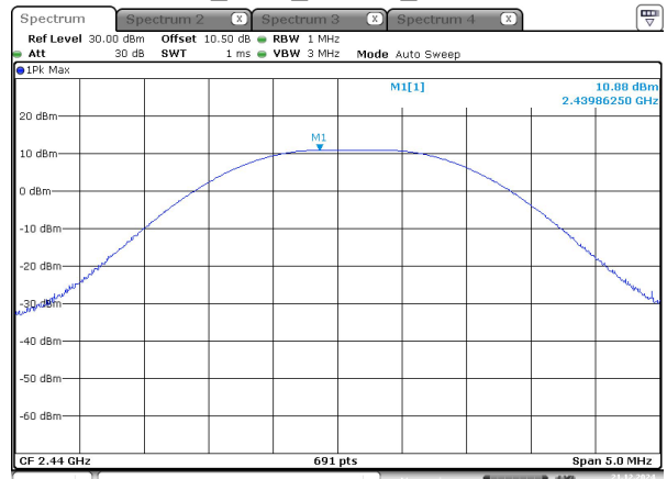
BLE_125k_Middle_Channel
