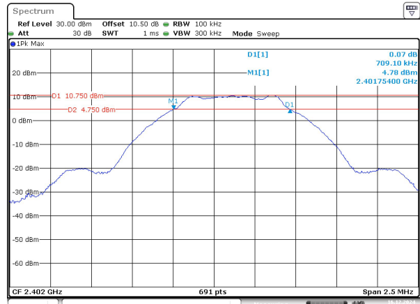
BLE_500k_Low_Channel
