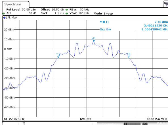
BLE_125k_Low_Channel
