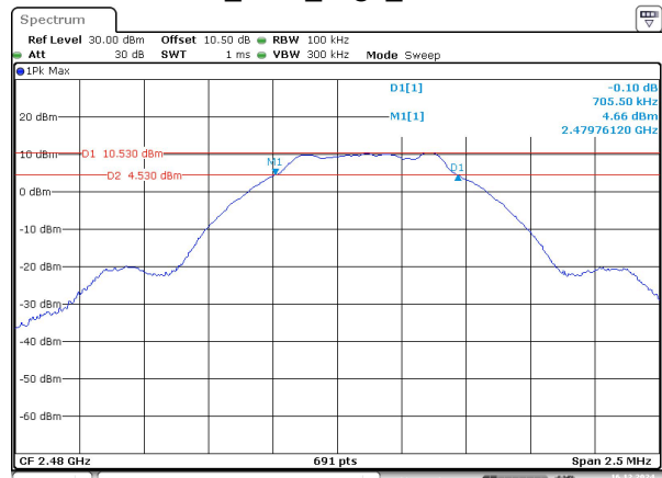
BLE_500k_High_Channel
