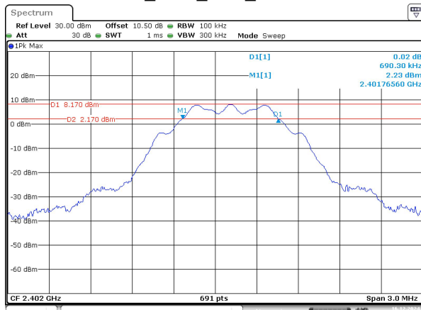
BLE_125k_Low_Channel
