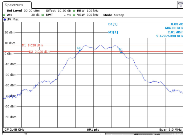
BLE_125k_High_Channel
