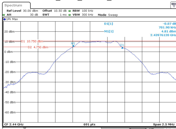
BLE_500k_Middle_Channel
