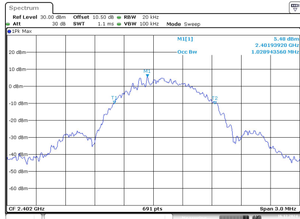
BLE_500k_Low_Channel
