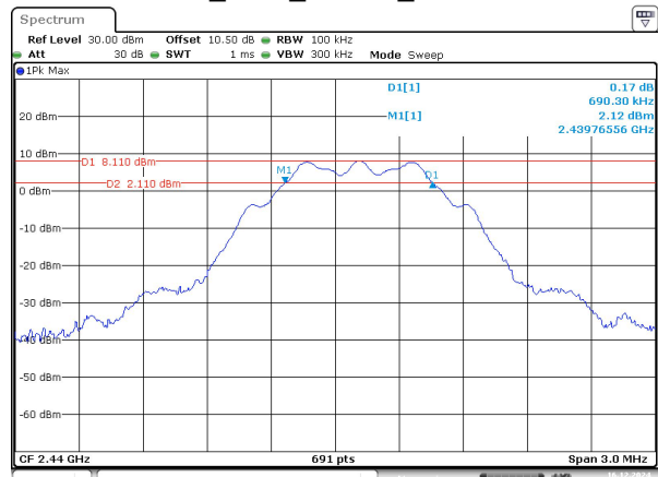
BLE_125k_Middle_Channel
