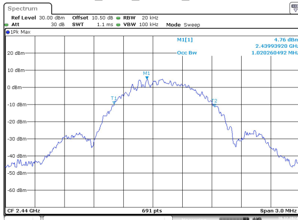
BLE_500k_Middle_Channel
