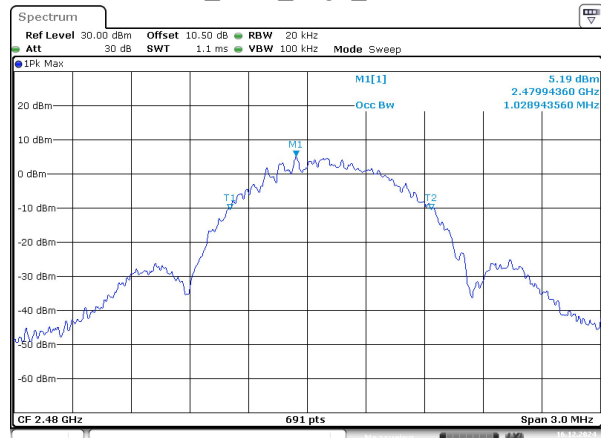
BLE_500k_High_Channel
