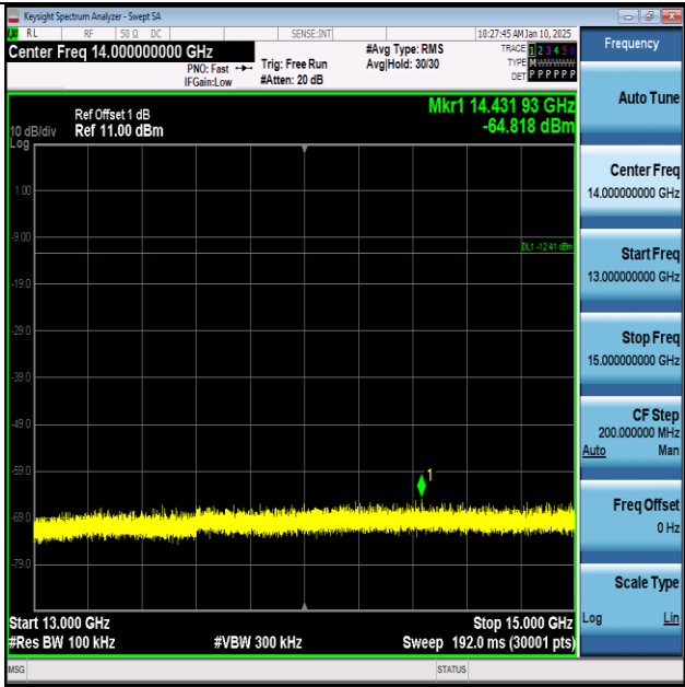
ZIGB-Ant1-2440-13000~15000-PASS
