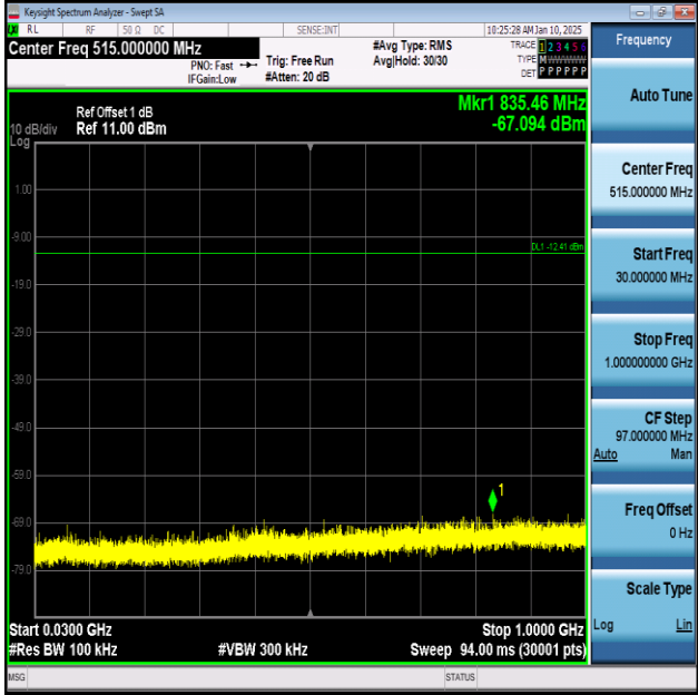
ZIGB-Ant1-2440-30~1000-PASS
