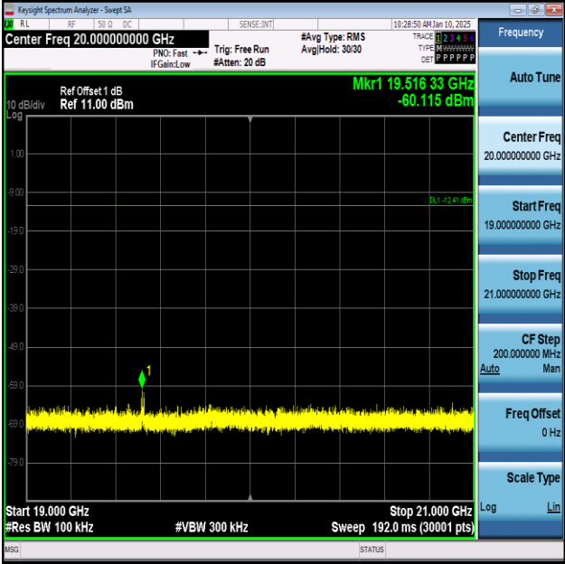
ZIGB-Ant1-2440-19000~21000-PASS
