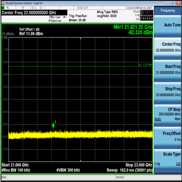
ZIGB-Ant1-2405-21000~23000-PASS
