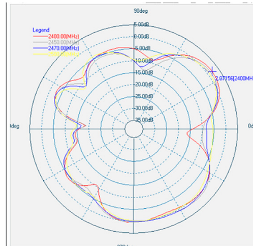
2.45GHz XZ Plane
