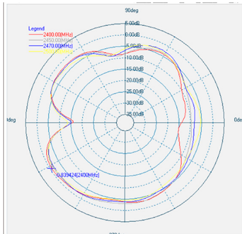
2.45GHz YZ Plane
