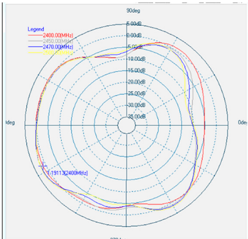
2.45GHz XY Plane
