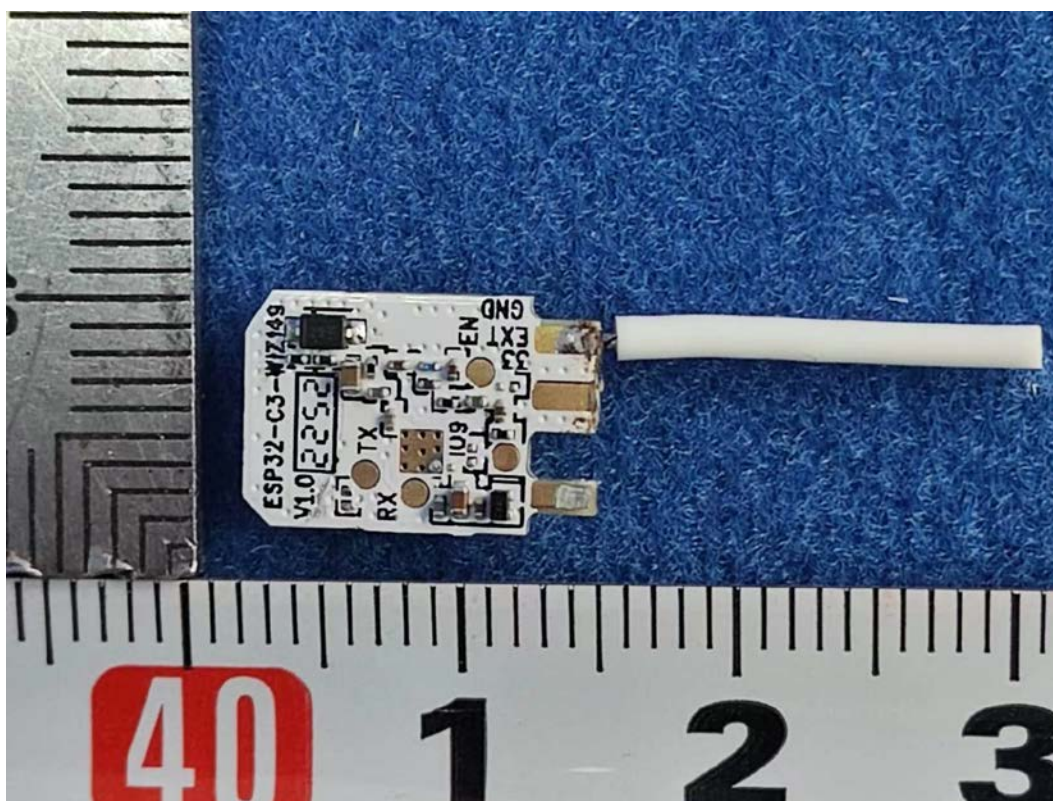
FIGURE 9 LED LAMP (M/N: 9290032676) RF BOARD BACK
