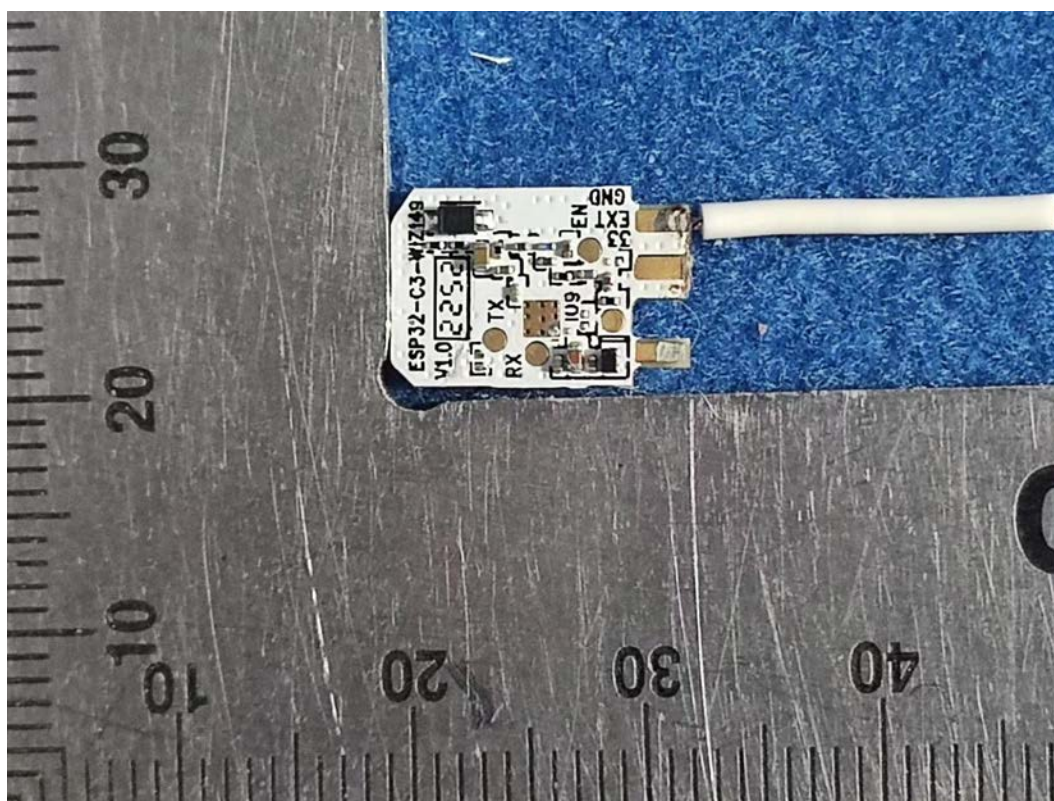
FIGURE 16 LED LAMP (M/N: 9290032675) ANTENNA
