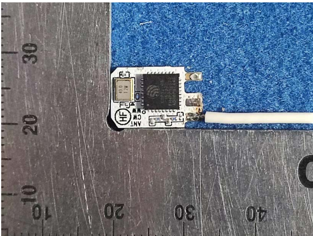
FIGURE 14 LED LAMP (M/N: 9290032675) RF BOARD FRONT
