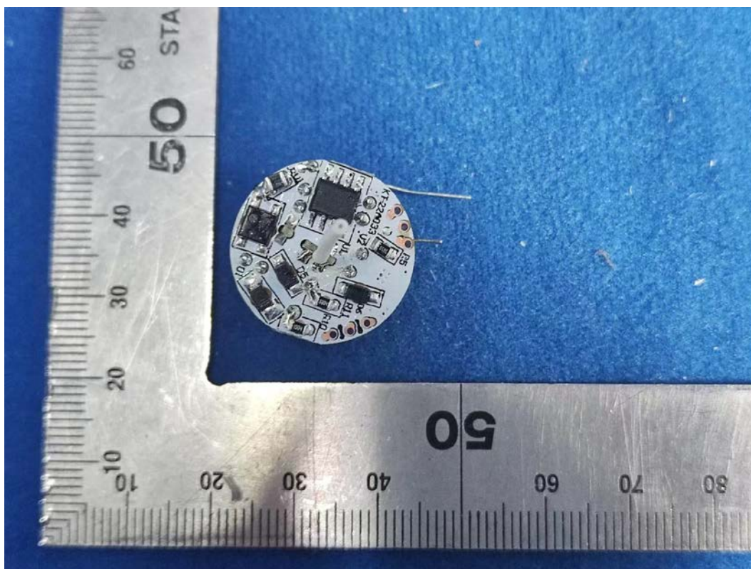
FIGURE 12 LED LAMP (M/N: 9290032675) MAINBOARD FRONT
