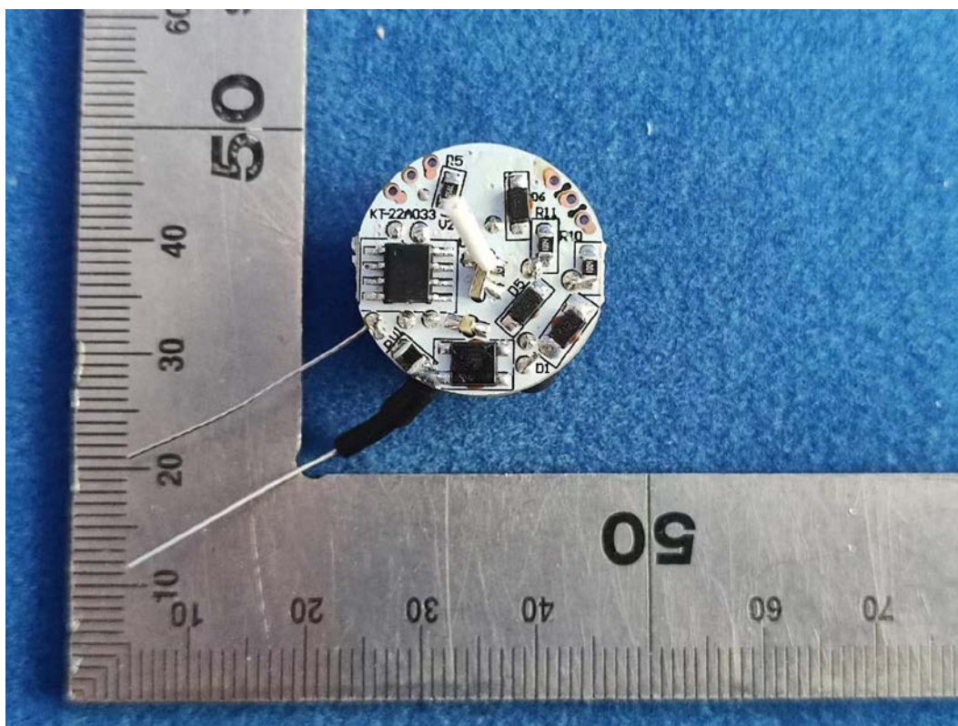
FIGURE 6 LED LAMP (M/N: 9290032676) MAINBOARD FRONT
