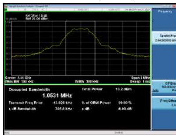
6dB Occupied Bandwidth
