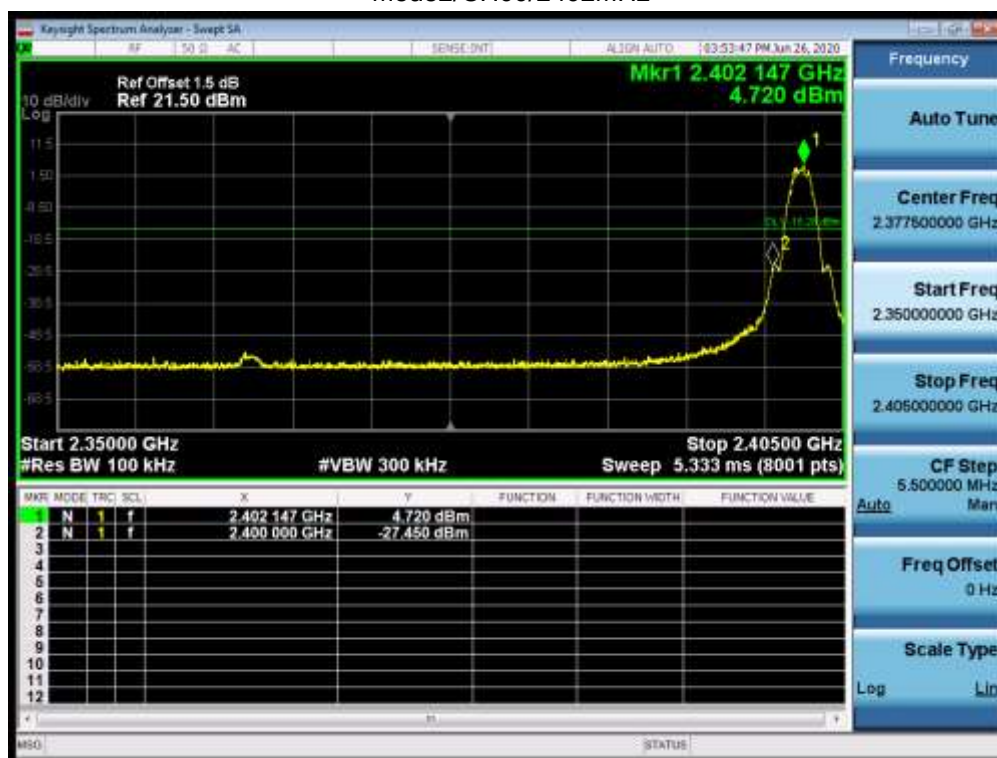
Mode2/CH00/2402MHz
