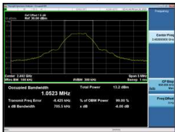
99% Occupied Bandwidth
