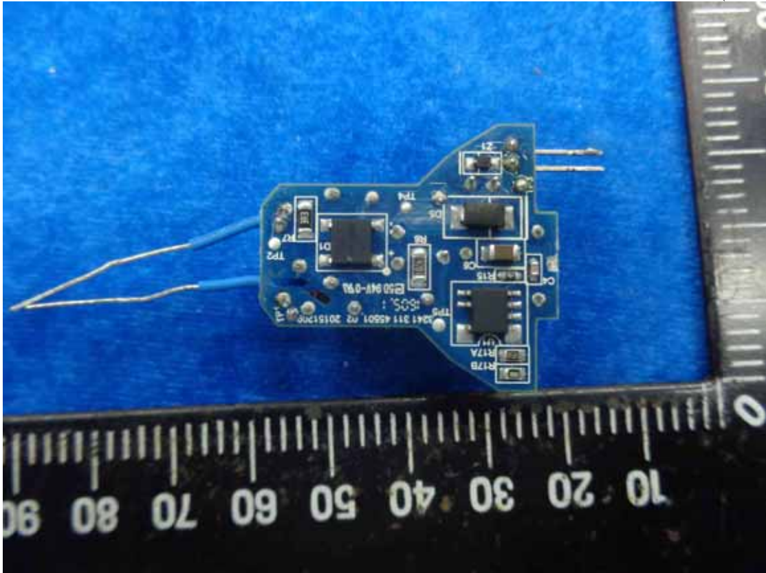
Figure 7 Power Board (Back View)
