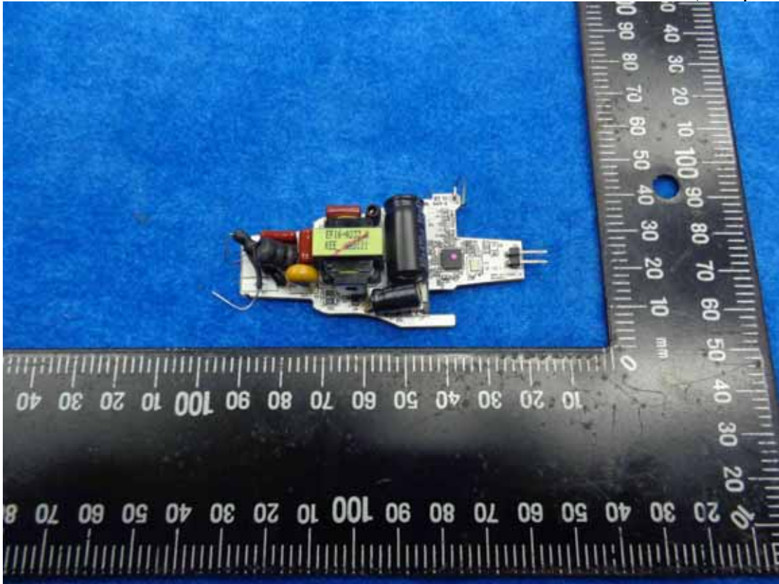
Figure 7 Power Board (Component Side)
