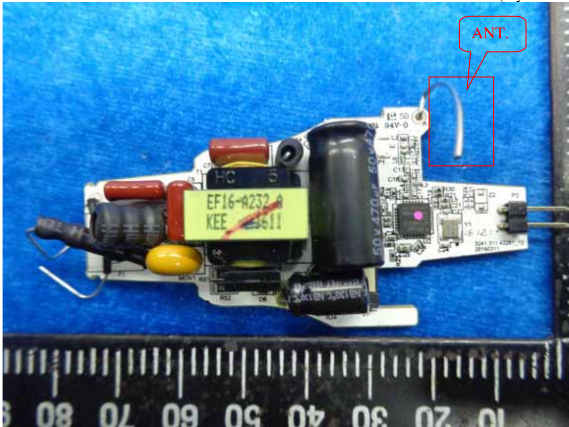
Figure 9 Wireless Board (crystal oscillator)
