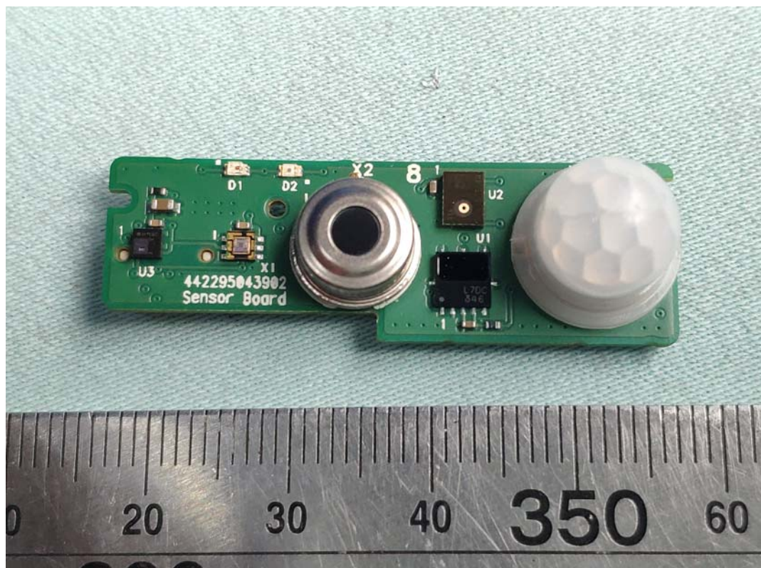
FIGURE 24 MISCELLANEOUS CONTROLS (M/N: SC1500/05) SENSOR BOARD (COMPONENT SIDE)
