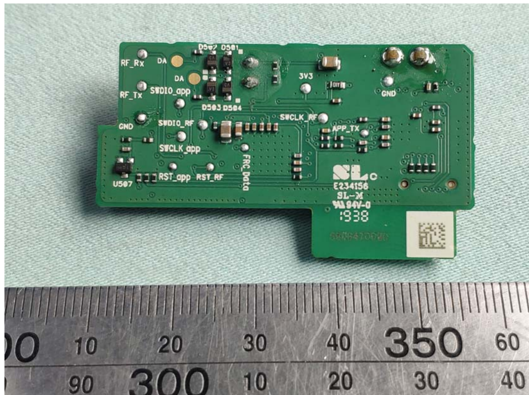
FIGURE 21 MISCELLANEOUS CONTROLS (M/N: SC1500/05) CONTROL BOARD (SOLDERED SIDE)
