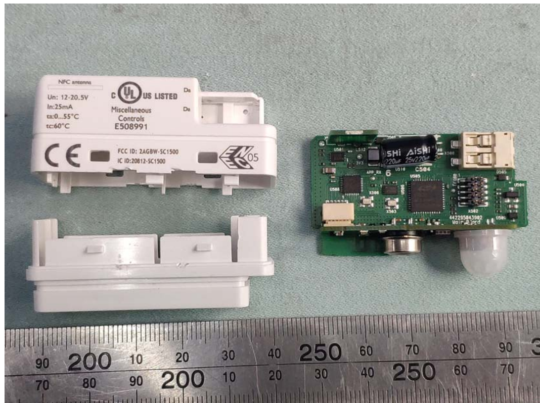
FIGURE 19 MISCELLANEOUS CONTROLS (M/N: SC1500/05) COVER REMOVED
