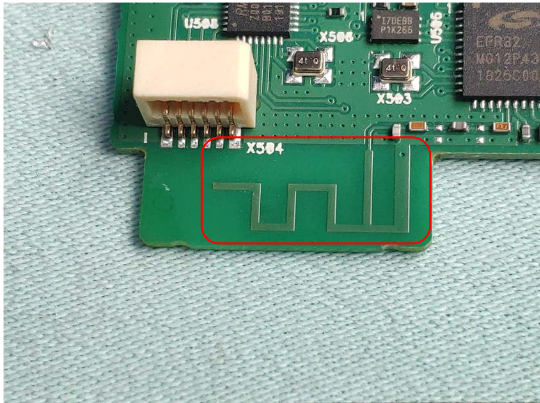
FIGURE 23 MISCELLANEOUS CONTROLS (M/N: SC1500/05) ANTENNA (GENERAL VIEW)
