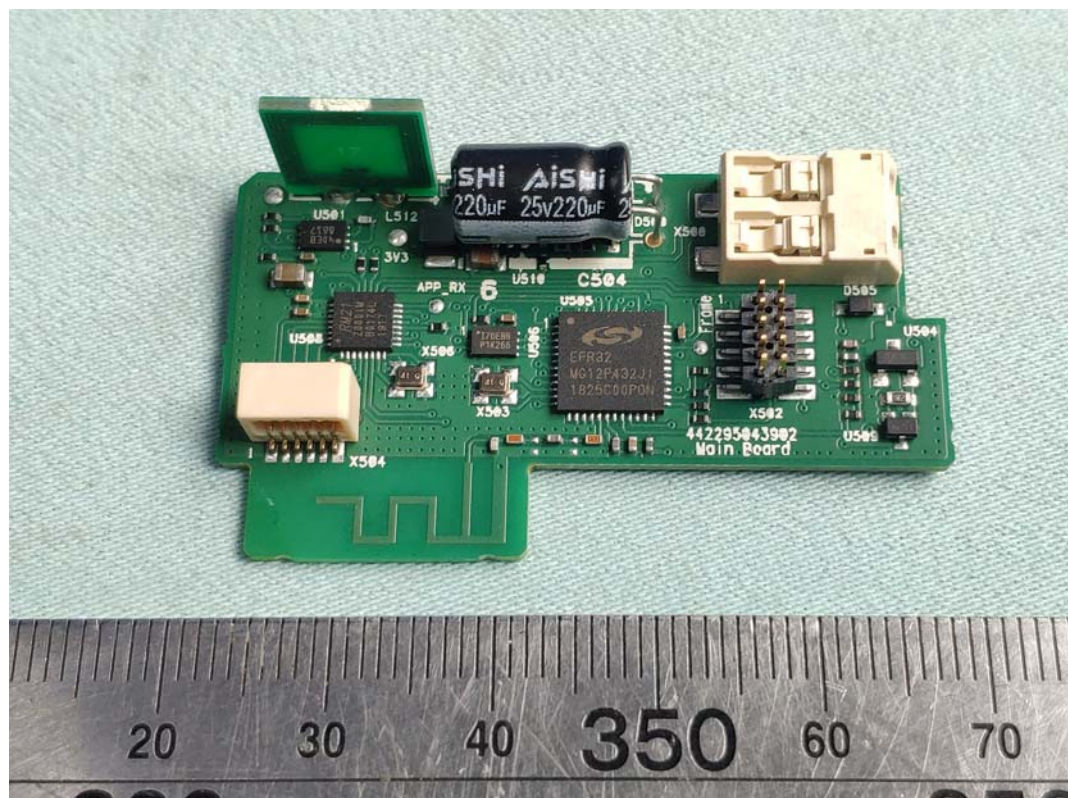
FIGURE 20 MISCELLANEOUS CONTROLS (M/N: SC1500/05) CONTROL BOARD (COMPONENT SIDE)
