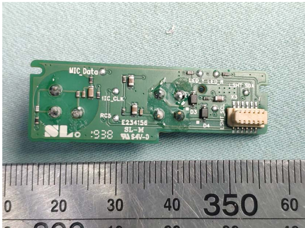
FIGURE 25 MISCELLANEOUS CONTROLS (M/N: SC1500/05) SENSOR BOARD (SOLDERED SIDE)
