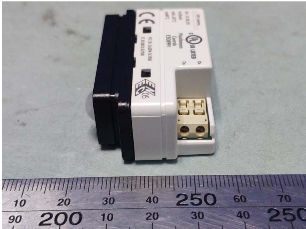
FIGURE 17 MISCELLANEOUS CONTROLS (M/N: SC1500/15) GENERAL APPEARANCE (RIGHT VIEW)
