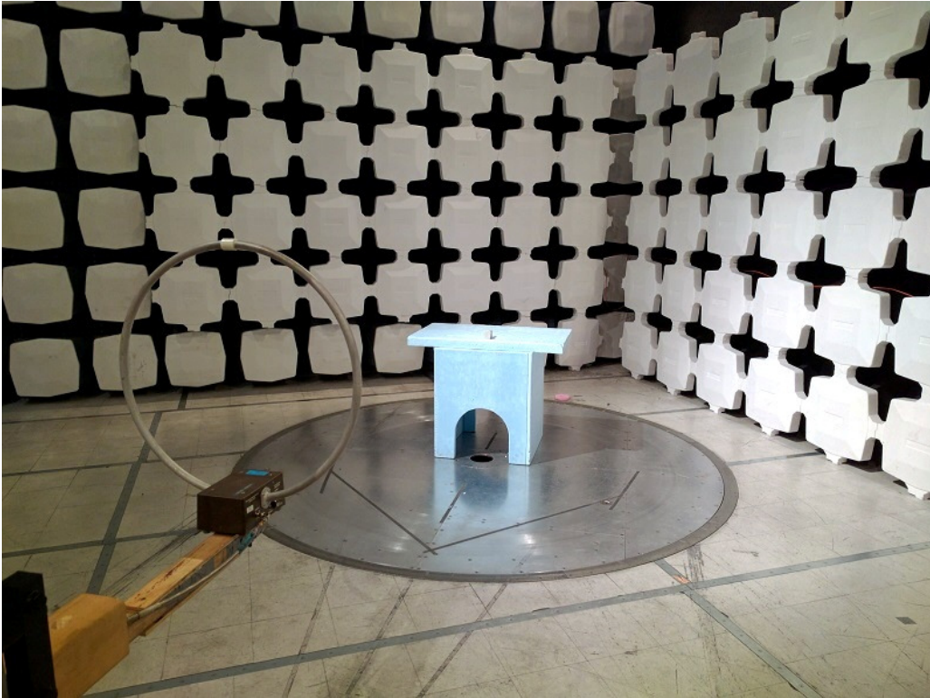
Figure 8: Radiated RF measurement, below 30 MHz, Position 2
