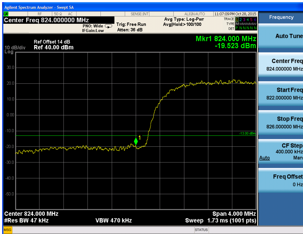
Fig.30 WCDMA Band V-CH4133 Band Edge Compliance HSUPA Subtest 5
