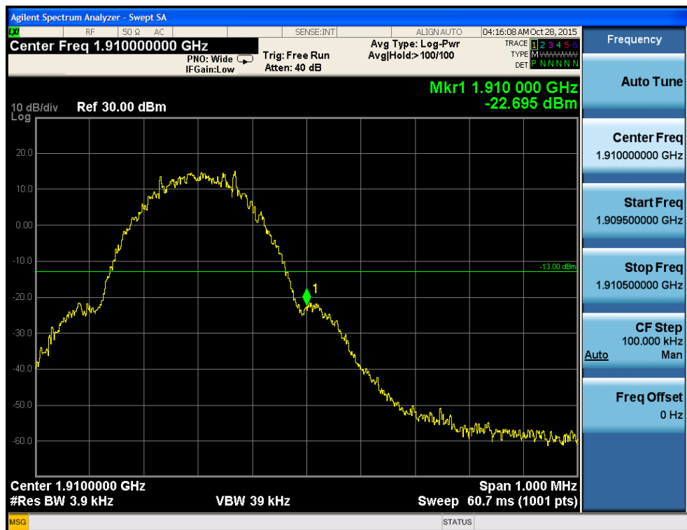
Fig.25 GSM1900-CH810 Band Edge Compliance
