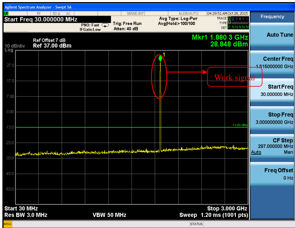
Fig.34 GSM1900 on Channel 661 30MHz~3GHz
