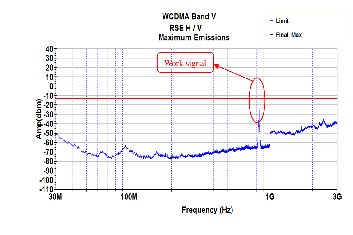
Fig.20 WCDMA Band V on Channel 4175 30MHz~3GHz
