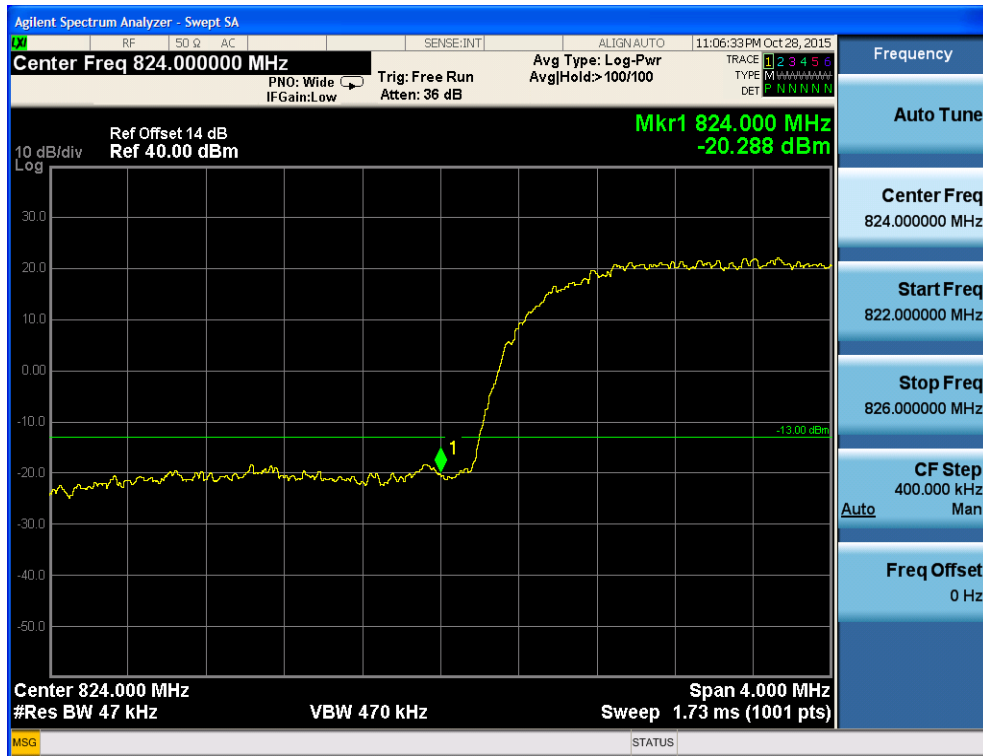
Fig.28 WCDMA Band V-CH4133 Band Edge Compliance HSDPA Subtest 1
