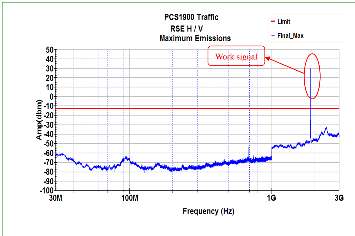
Fig.18 GSM1900 on Channel 661 30MHz~3GHz
