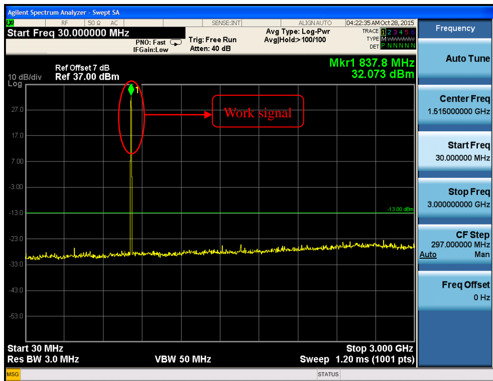
Fig.32 GSM850 on Channel 189 30MHz~3GHz
