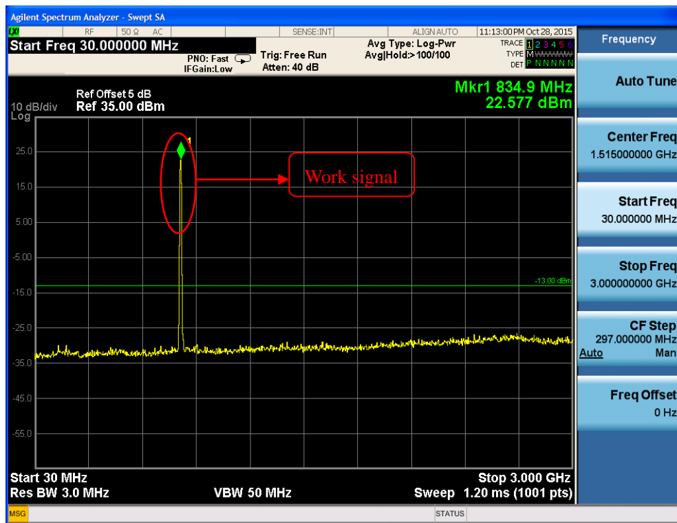
Fig.36 WCDMA Band V on Channel 4175 30MHz~3GHz
