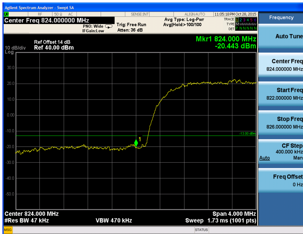
Fig.26 WCDMA Band V-CH4133 Band Edge Compliance
