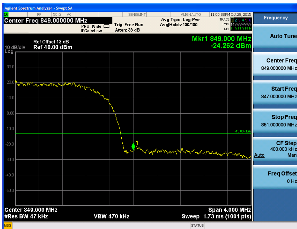
Fig.27 WCDMA Band V-CH4232 Band Edge Compliance
