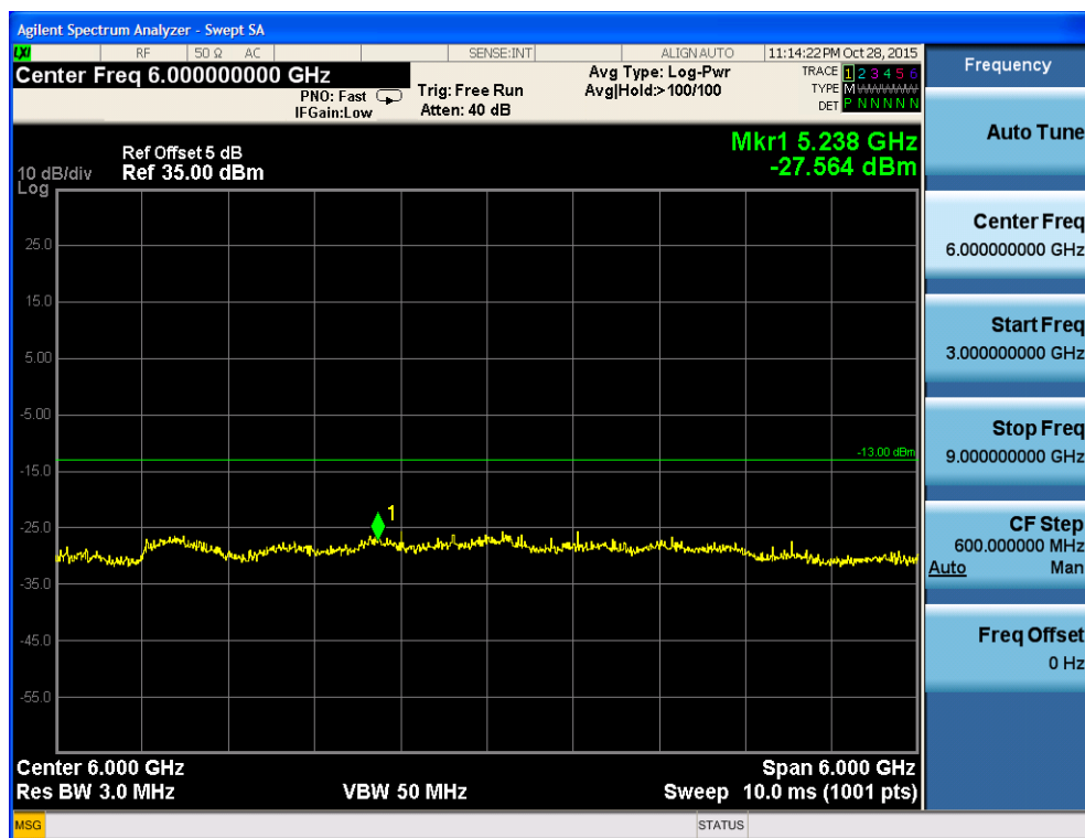
Fig.37 WCDMA Band V on Channel 4175 3GHz~9GHz
