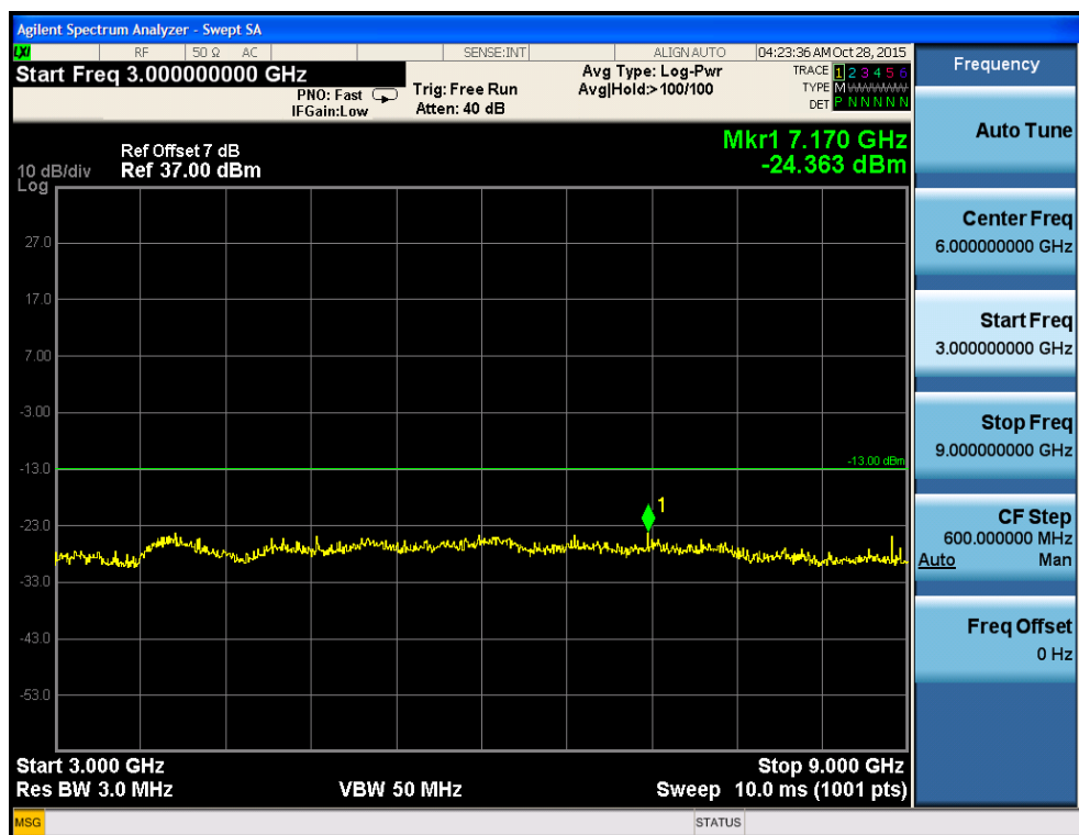
Fig.33 GSM850 on Channel 189 3GHz~9GHz
