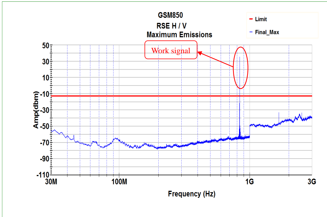
Fig.16 GSM850 on Channel 189 30MHz~3GHz
