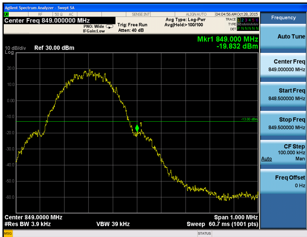
Fig.23 GSM850-CH251 Band Edge Compliance
