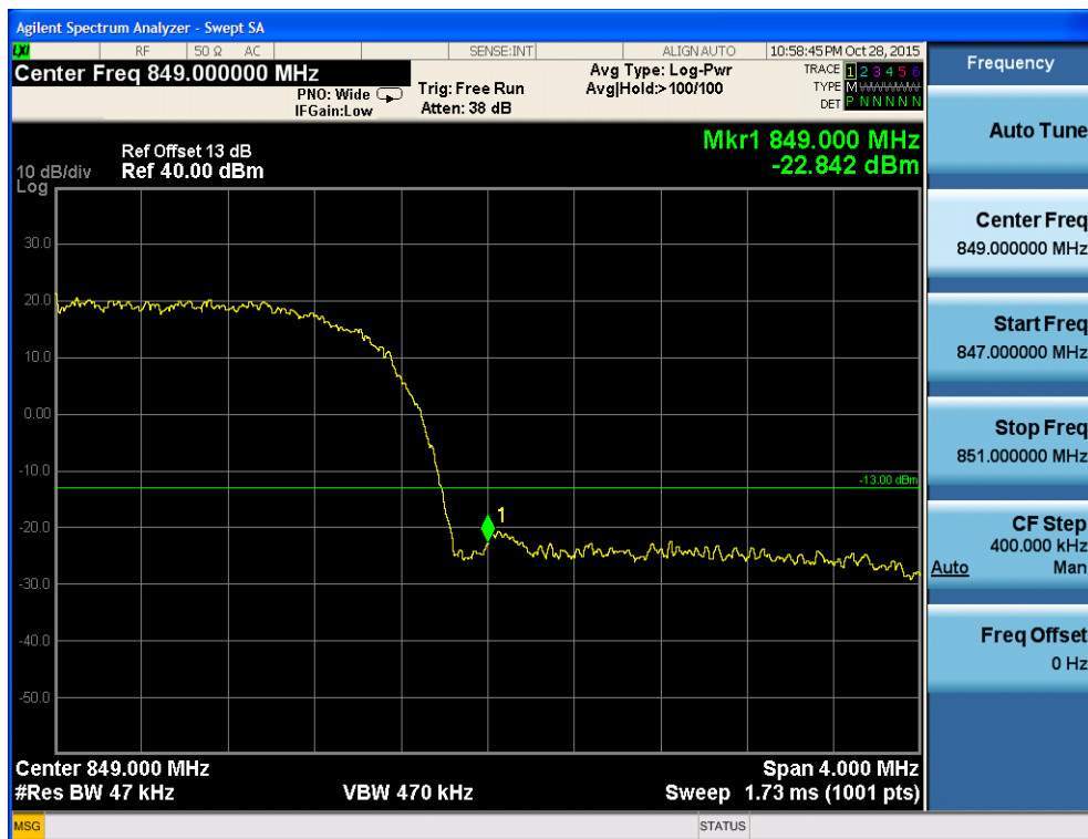
Fig.31 WCDMA Band V-CH4232 Band Edge Compliance HSUPA Subtest 5
