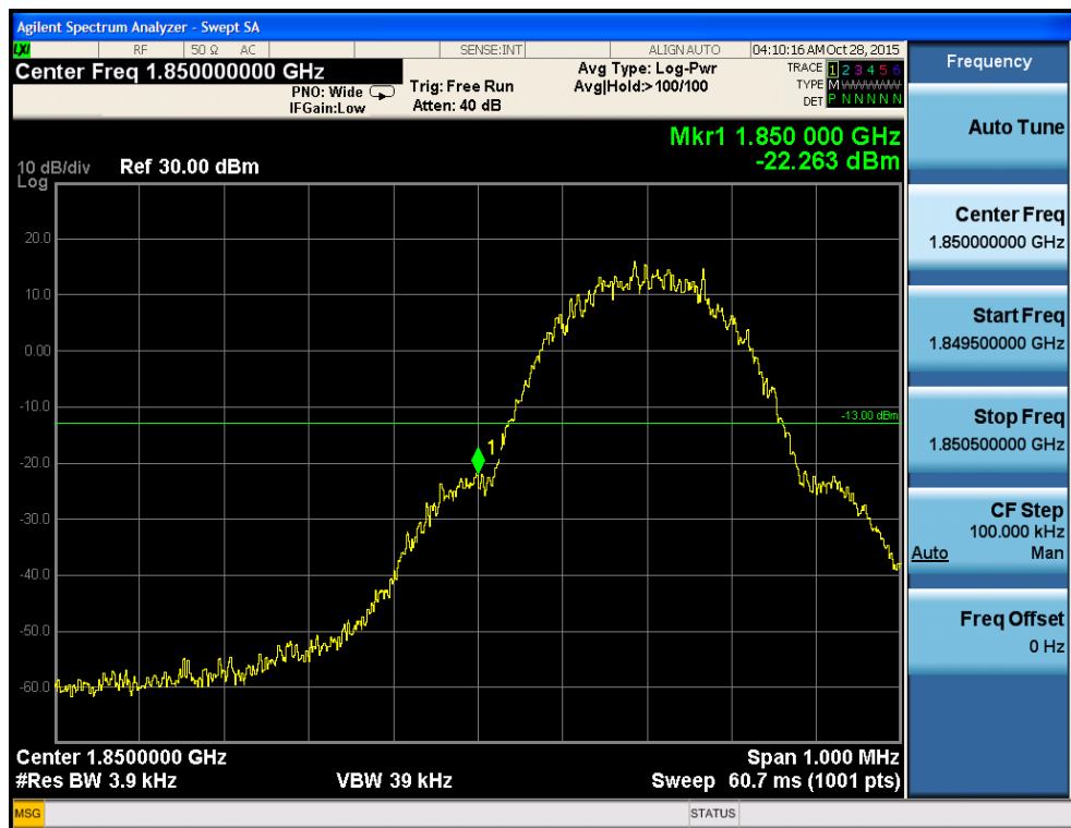
Fig.24 GSM1900-CH512 Band Edge Compliance
