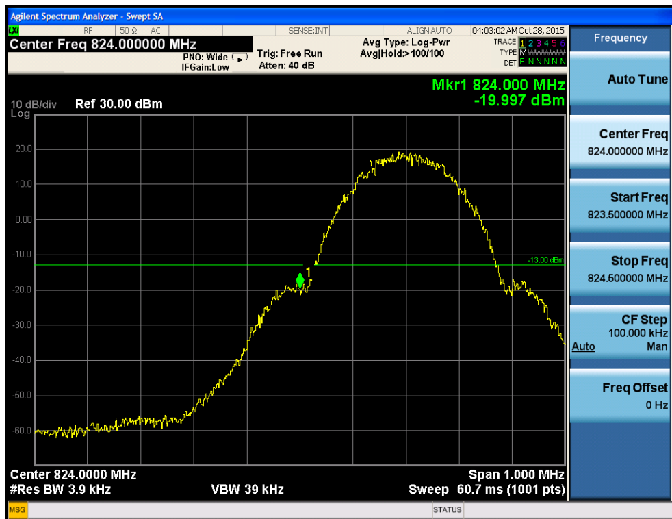
Fig.22 GSM850-CH128 Band Edge Compliance
