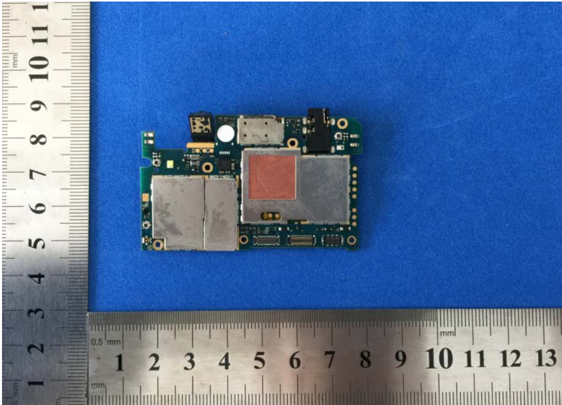
Main board with shielding Front View
