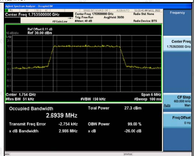
Middle Channel
