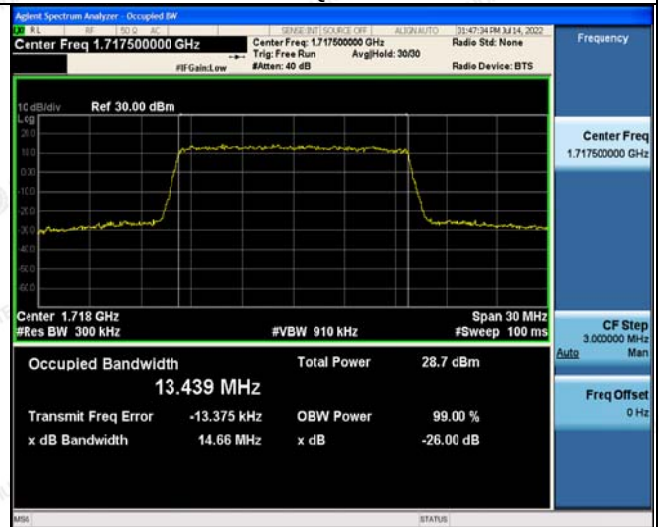
16QAM
