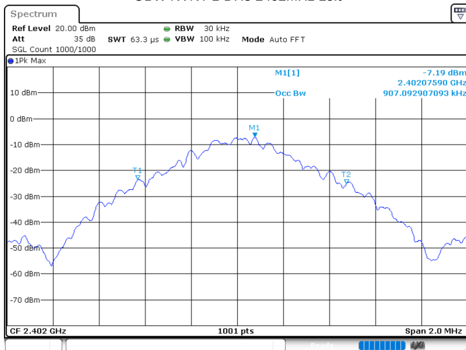
OBW NVNT 1-DH5 2402MHz Left
