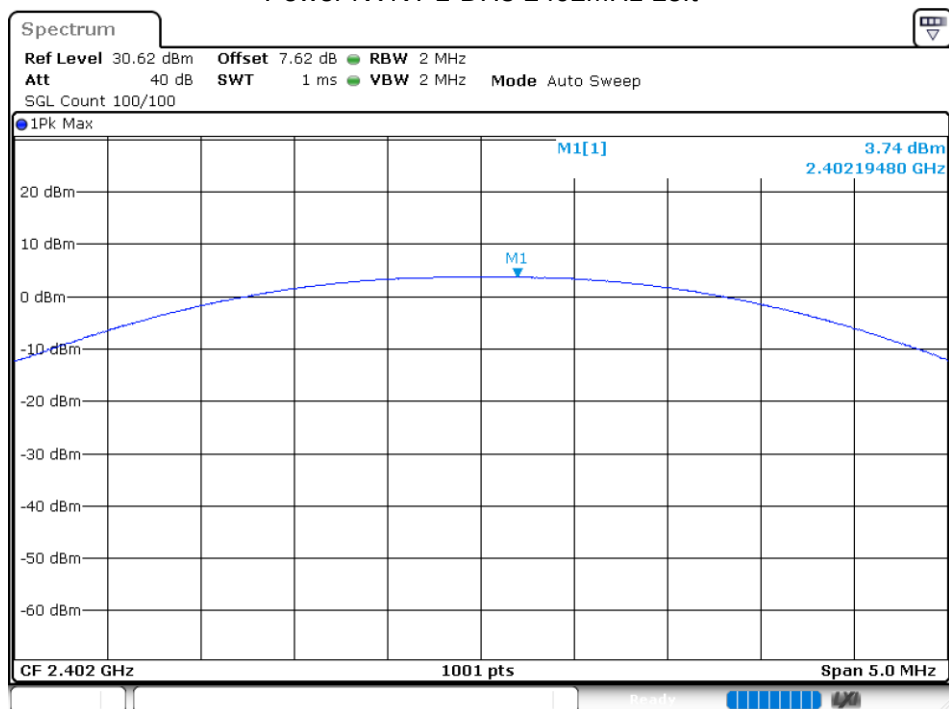
Power NVNT 1-DH5 2402MHz Left
