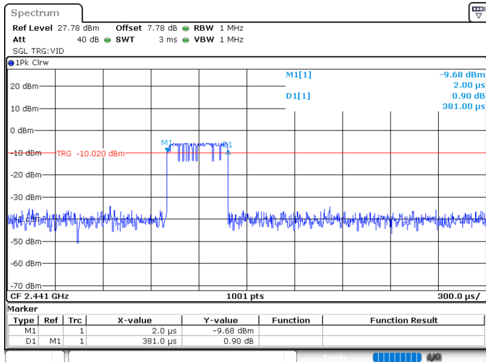
Dwell NVNT 1-DH1 2441MHz Left
