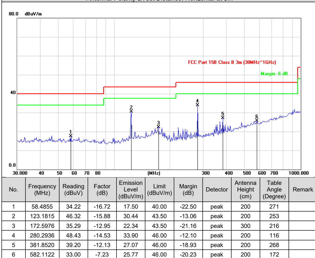
Antennal Polarity & Test Distance: Horizontal at 3m
