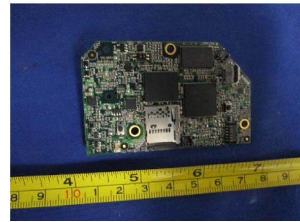
PCBA 1 RearView
