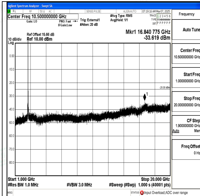
Band38_20MHz_16QAM_38000_1RB#0_1000~20000_1 000~20000
