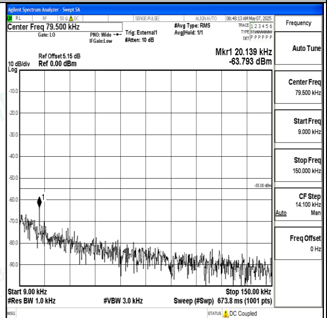
Band38_15MHz_16QAM_38000_1RB#0_0.009~0.15_0. 009~0.15
