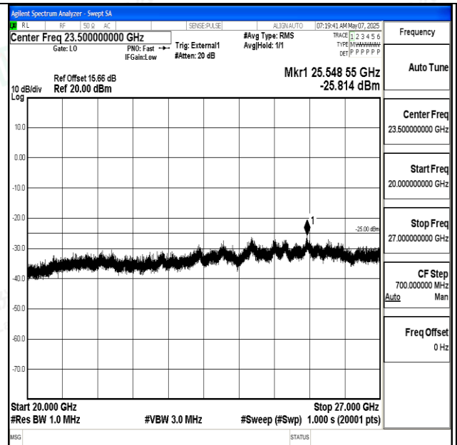
Band38_20MHz_16QAM_38000_1RB#0_20000~27000_ 20000~27000
