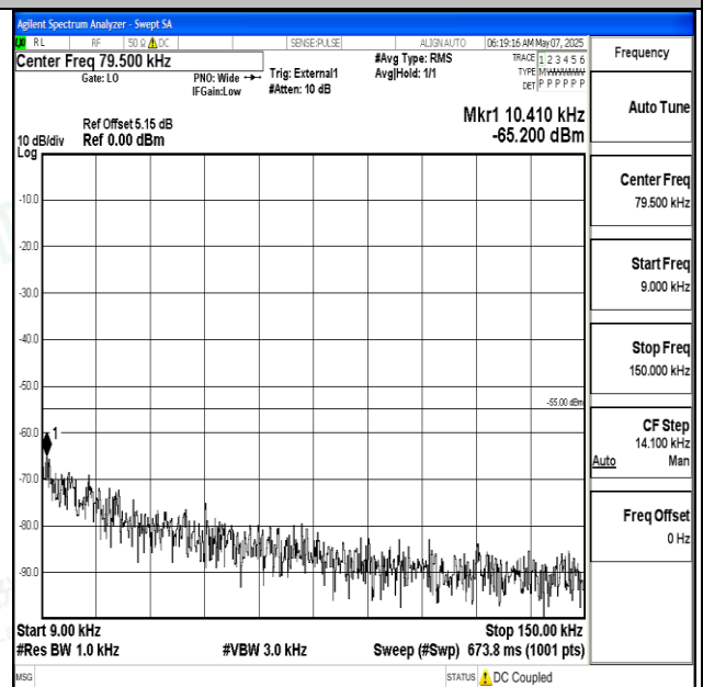
Band38_10MHz_16QAM_38200_1RB#0_0.009~0.15_0. 009~0.15
