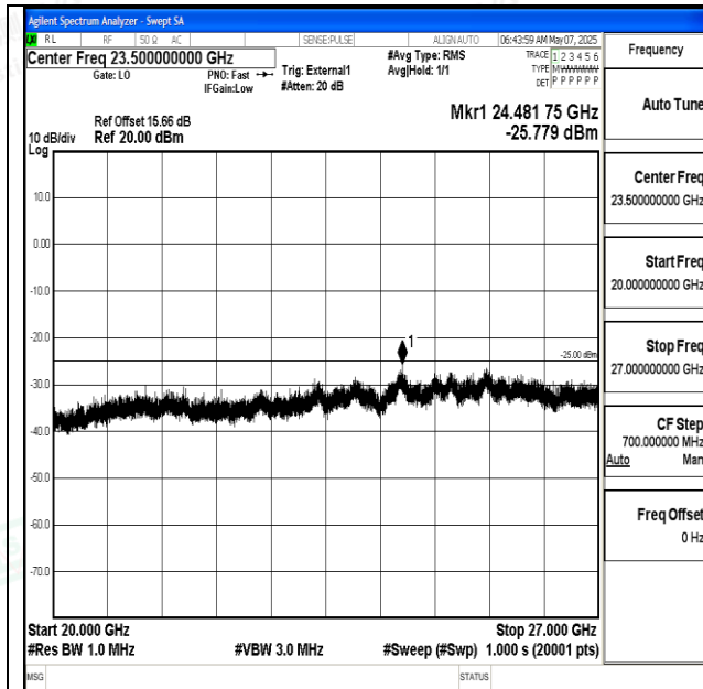
Band38_15MHz_QPSK_37825_1RB#0_20000~27000_2 0000~27000
