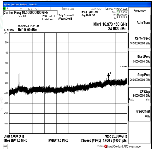
Band38_15MHz_QPSK_38000_1RB#0_1000~20000_10 00~20000
