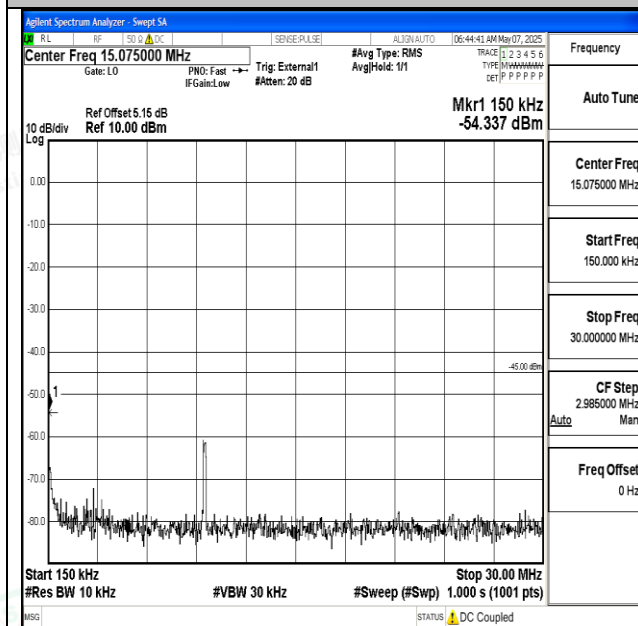
Band38_15MHz_16QAM_37825_1RB#0_0.15~30_0.15~ 30
