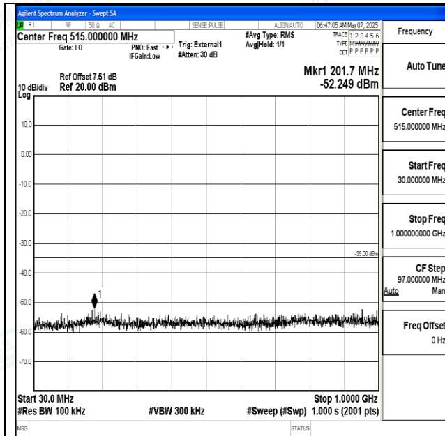
Band38_15MHz_QPSK_38000_1RB#0_30~1000_30~10 00
