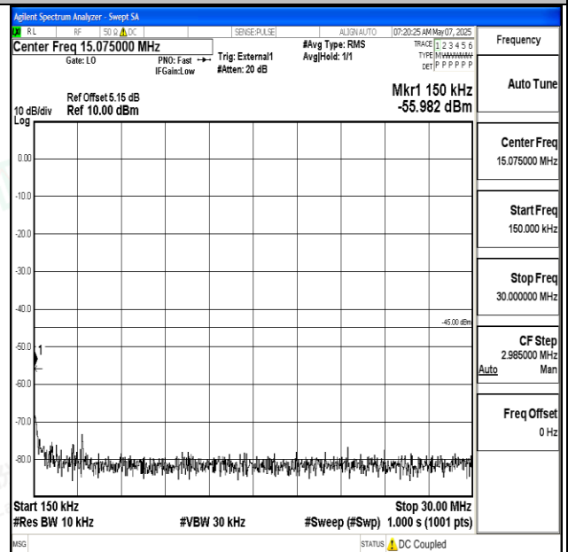
Band38_20MHz_QPSK_38150_1RB#0_0.15~30_0.15~3 0
