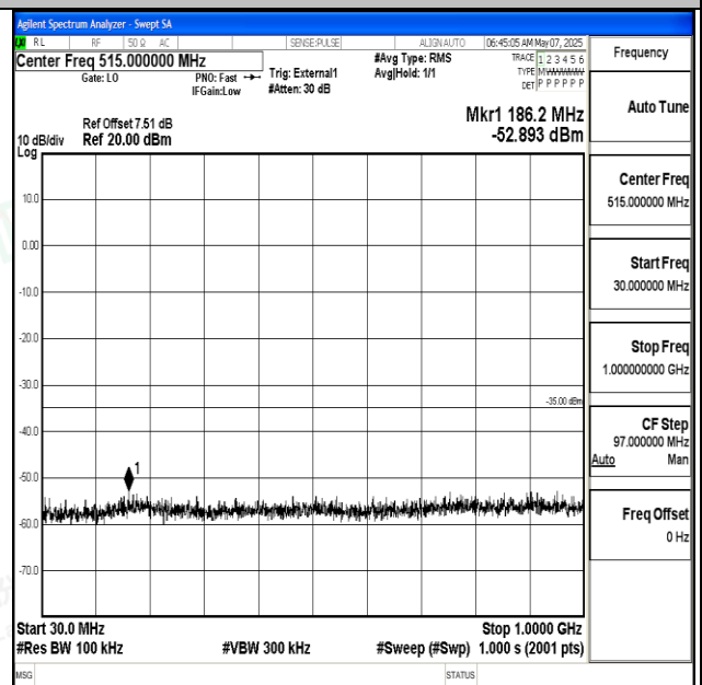
Band38_15MHz_16QAM_37825_1RB#0_30~1000_30~1 000
