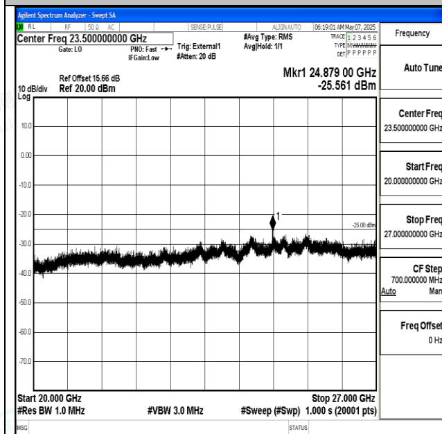
Band38_10MHz_QPSK_38200_1RB#0_20000~27000_2 0000~27000
