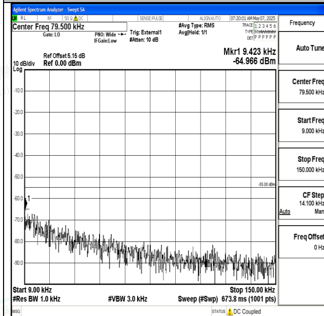
Band38_20MHz_QPSK_38150_1RB#0_0.009~0.15_0.00 9~0.15
