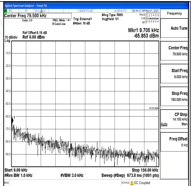
Band38_15MHz_16QAM_37825_1RB#0_0.009~0.15_0. 009~0.15
