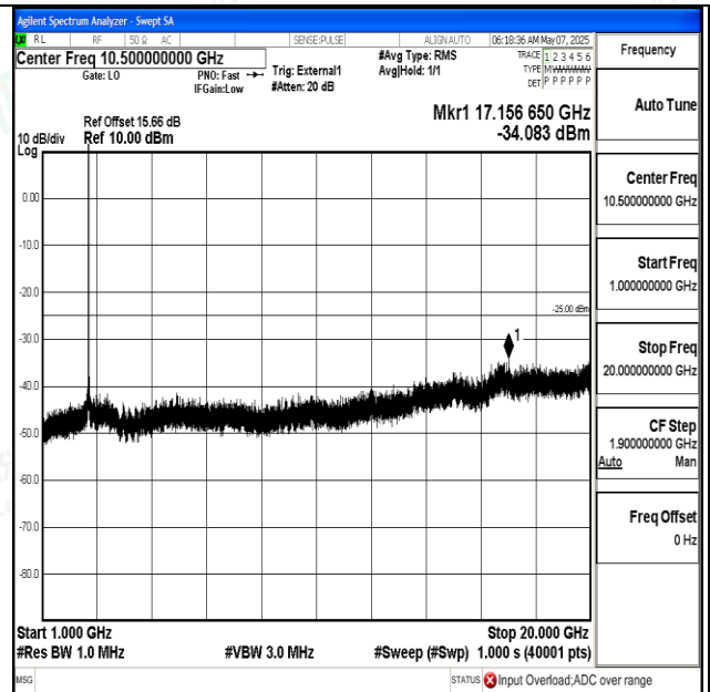
Band38_10MHz_QPSK_38200_1RB#0_1000~20000_10 00~20000
