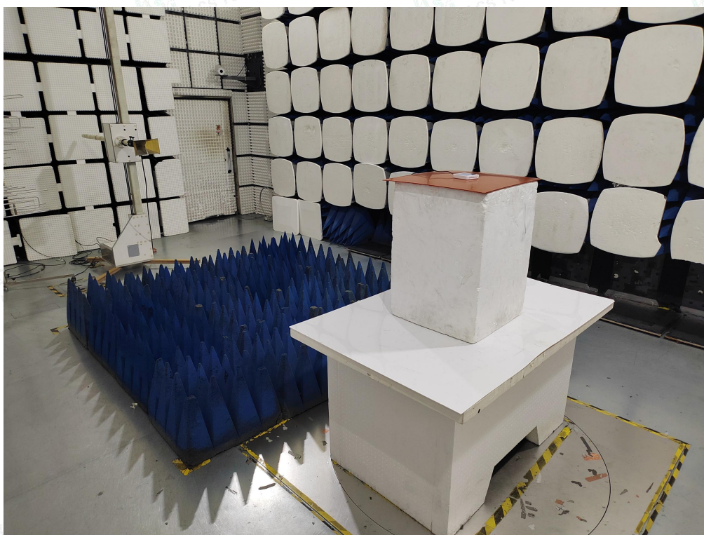
Radiated Emissions Measurement (Above 1GHz)
