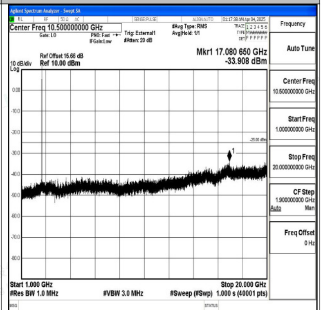
Band41_10MHz_QPSK_40620_1RB#0_1000~20000_10 00~20000
