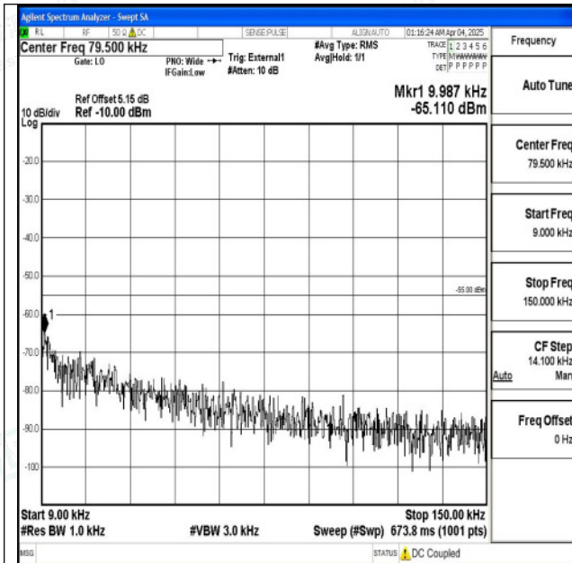
Band41_10MHz_QPSK_40620_1RB#0_0.009~0.15_0.00 9~0.15
