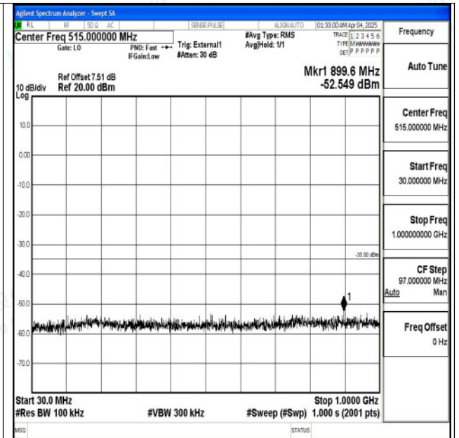
Band41_15MHz_16QAM_40620_1RB#0_30~1000_30~1000
