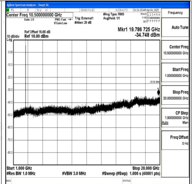
Band41_15MHz_QPSK_40620_1RB#0_1000~20000_1000~20000
