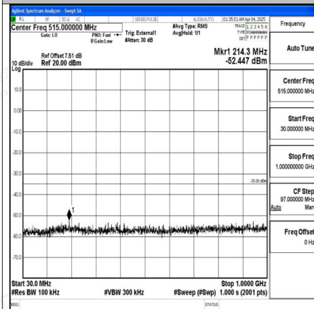
Band41_15MHz_QPSK_41515_1RB#0_30~1000_30~10 00
