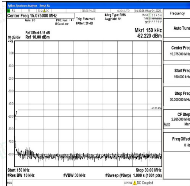
Band41_15MHz_16QAM_40620_1RB#0_0.15~30_0.15~30
