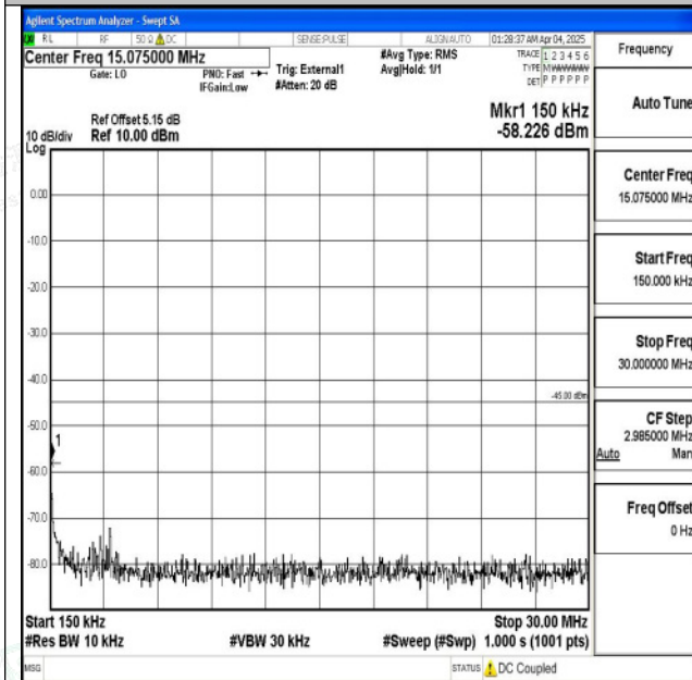
Band41_15MHz_16QAM_39725_1RB#0_0.15~30_0.15~ 30
