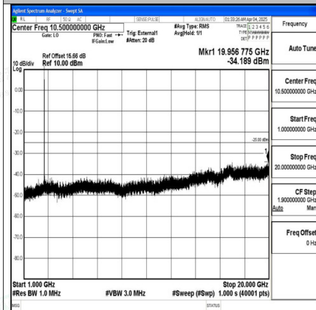
Band41_15MHz_16QAM_40620_1RB#0_1000~20000_1000~20000
