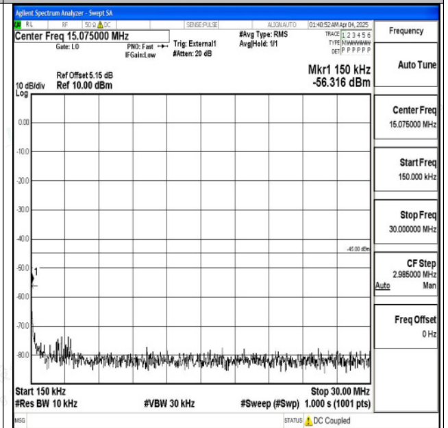
Band41_20MHz_QPSK_39750_1RB#0_0.15~30_0.15~3 0
