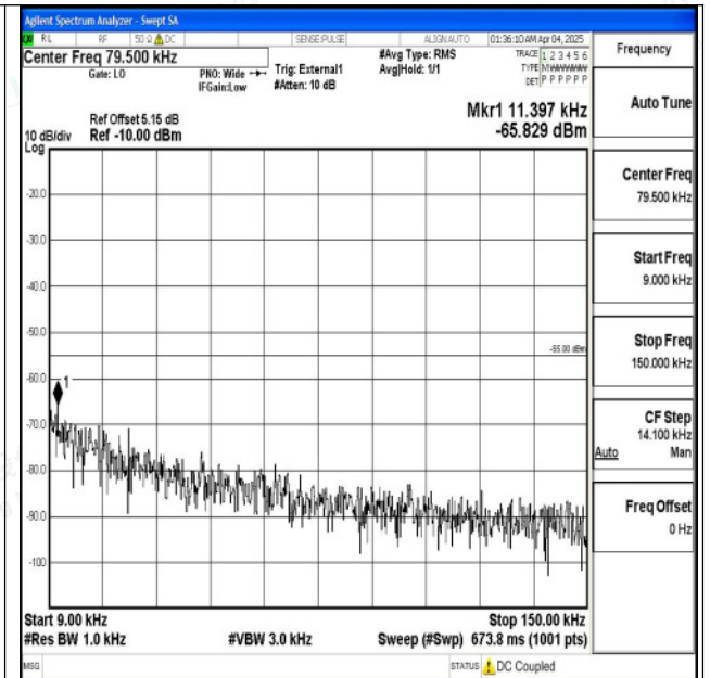
Band41_15MHz_16QAM_41515_1RB#0_0.009~0.15_0. 009~0.15
