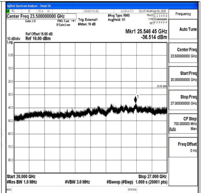
Band41_15MHz_16QAM_41515_1RB#0_20000~27000_ 20000~27000
