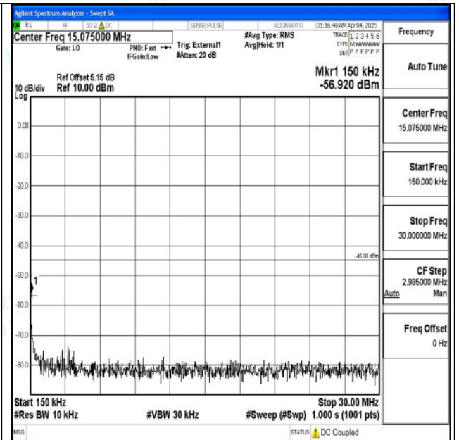
Band41_10MHz_QPSK_40620_1RB#0_0.15~30_0.15~3 0
