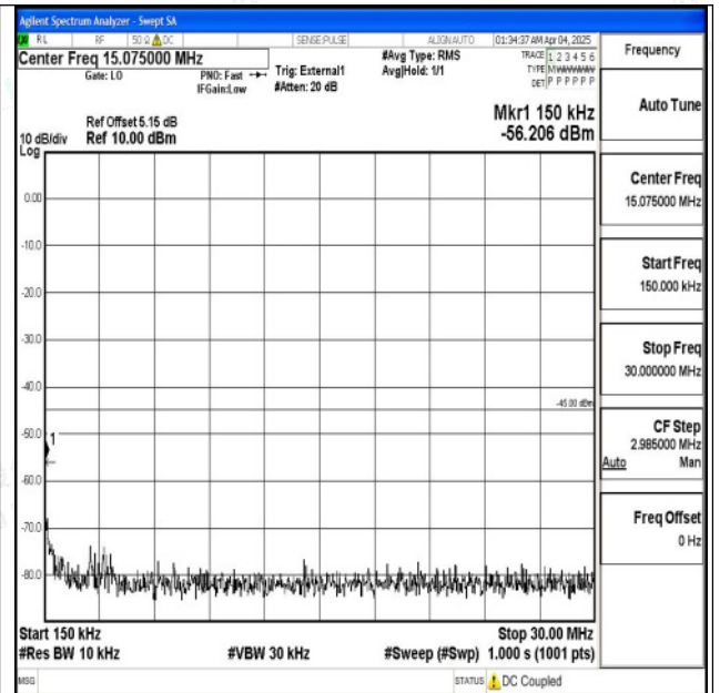
Band41_15MHz_QPSK_41515_1RB#0_0.15~30_0.15~3 0
