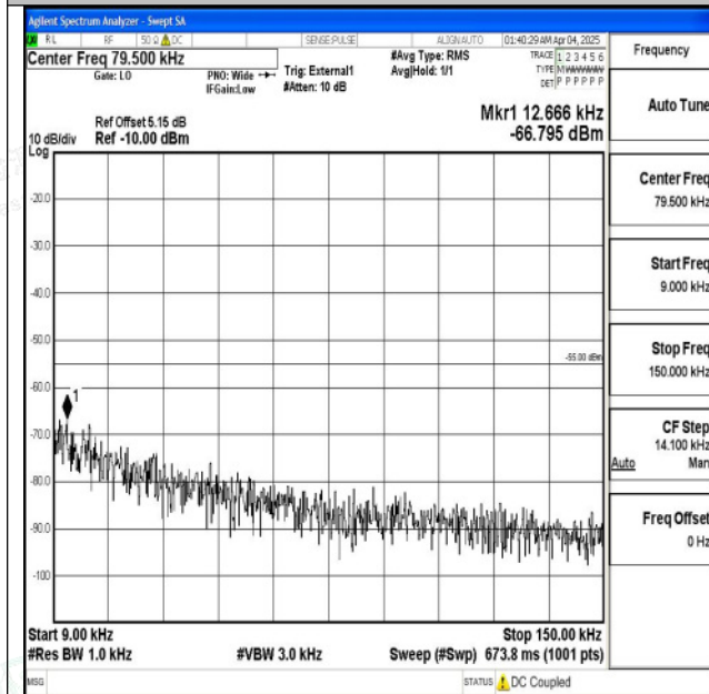
Band41_20MHz_QPSK_39750_1RB#0_0.009~0.15_0.00 9~0.15
