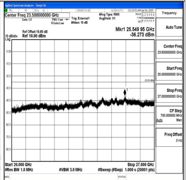
Band41_10MHz_16QAM_41540_1RB#0_20000~27000_20000~27000
