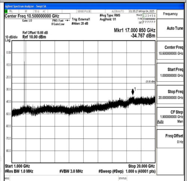
Band41_15MHz_QPSK_41515_1RB#0_1000~20000_10 00~20000
