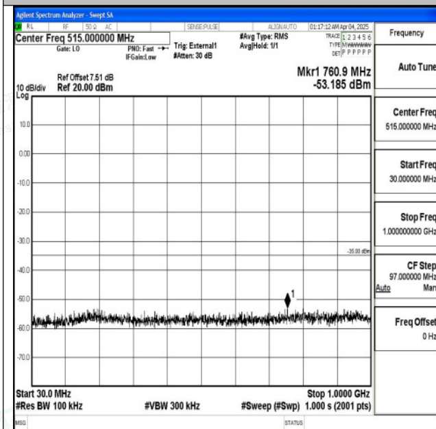
Band41_10MHz_QPSK_40620_1RB#0_30~1000_30~10 00
