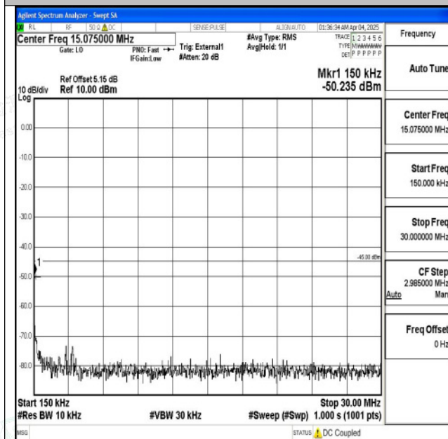
Band41_15MHz_16QAM_41515_1RB#0_0.15~30_0.15~ 30
