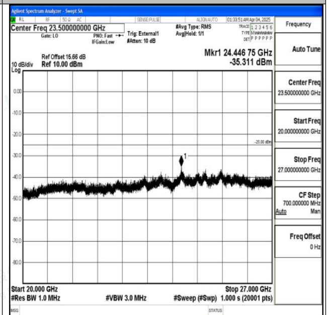
Band41_15MHz_16QAM_40620_1RB#0_20000~27000_20000~27000
