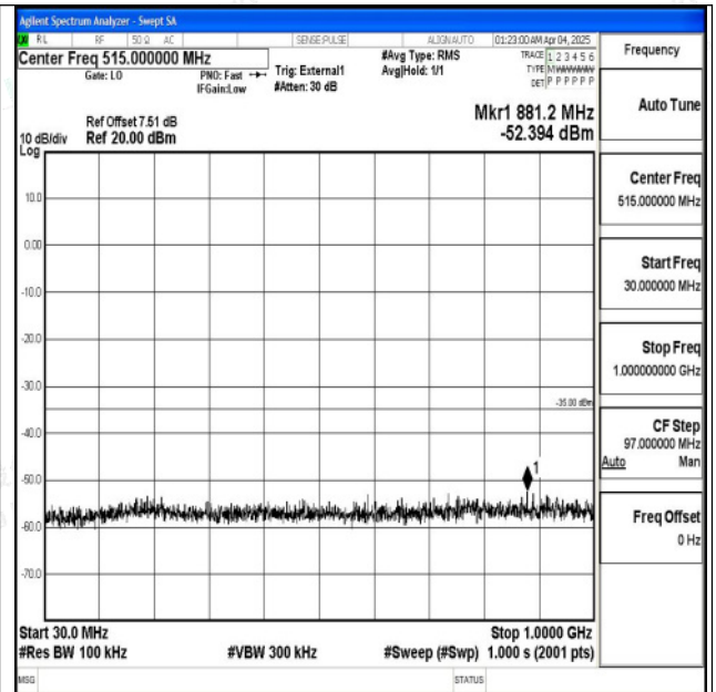
Band41_10MHz_16QAM_41540_1RB#0_30~1000_30~1000
