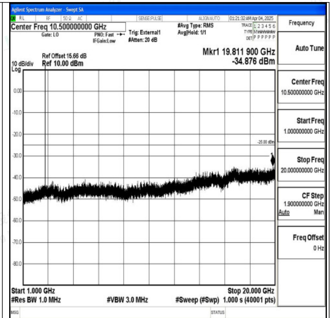
Band41_10MHz_QPSK_41540_1RB#0_1000~20000_1000~20000
