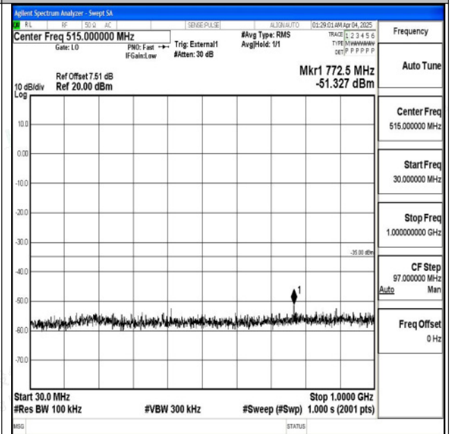
Band41_15MHz_16QAM_39725_1RB#0_30~1000_30~1 000
