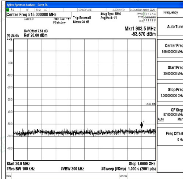
Band41_15MHz_QPSK_40620_1RB#0_30~1000_30~1000
