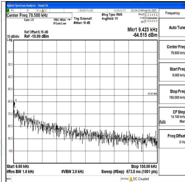
Band41_15MHz_QPSK_41515_1RB#0_0.009~0.15_0.00 9~0.15
