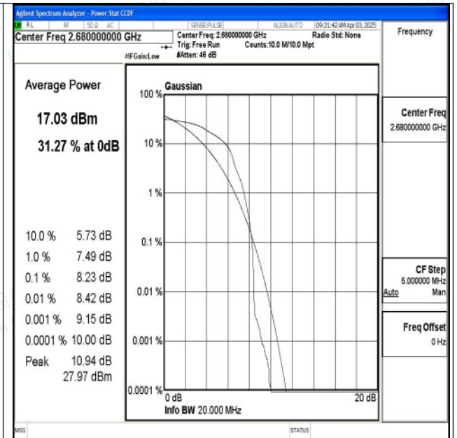
Band41-20MHz-16QAM-41490-1RB#0-PASS
