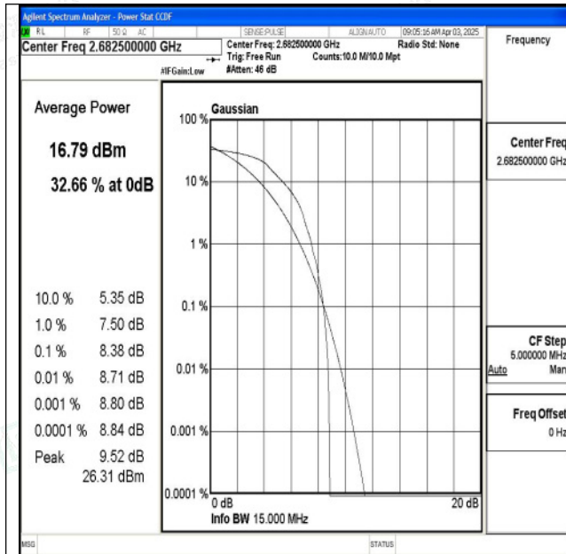
Band41-15MHz-QPSK-41515-1RB#0-PASS
