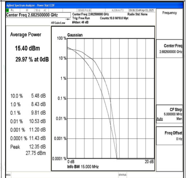
Band41-15MHz-16QAM-41515-75RB#0-PASS
