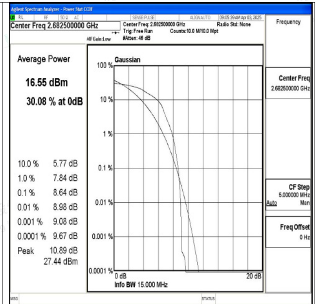
Band41-15MHz-16QAM-41515-1RB#0-PASS
