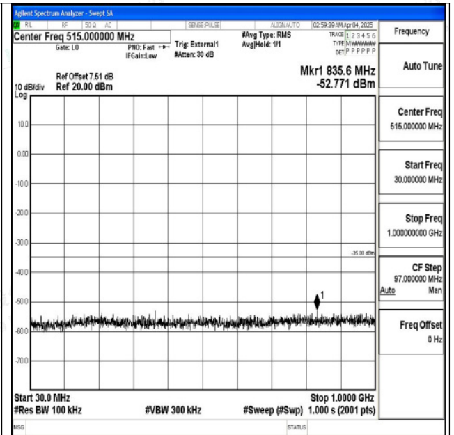
Band38_20MHz_16QAM_38150_1RB#0_30~1000_30~1000
