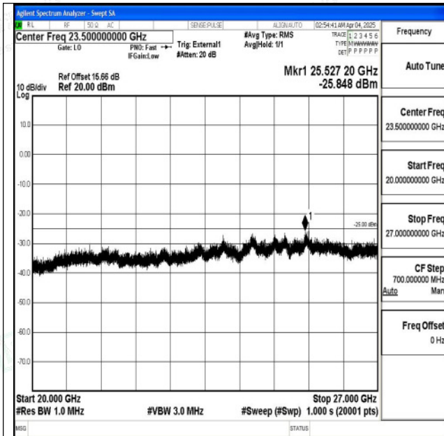
Band38_20MHz_QPSK_38000_1RB#0_20000~27000_2 0000~27000
