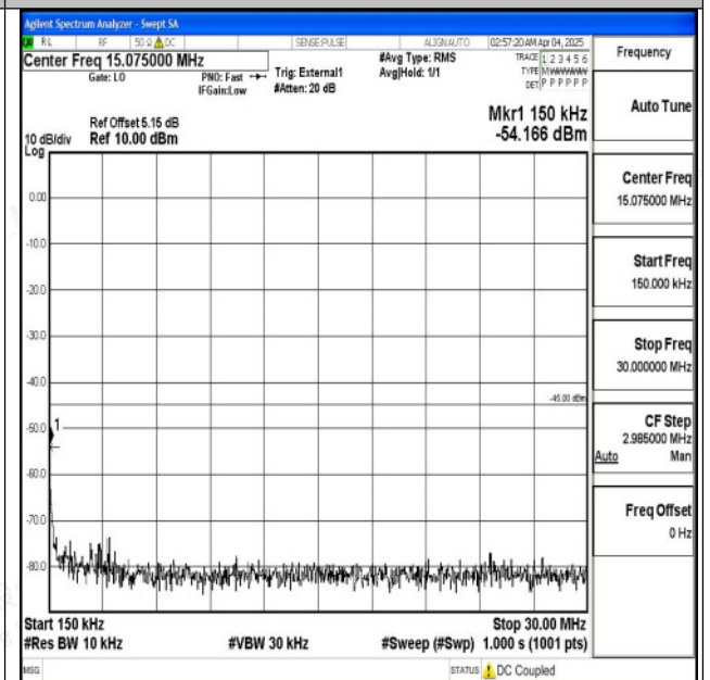
Band38_20MHz_QPSK_38150_1RB#0_0.15~30_0.15~3 0
