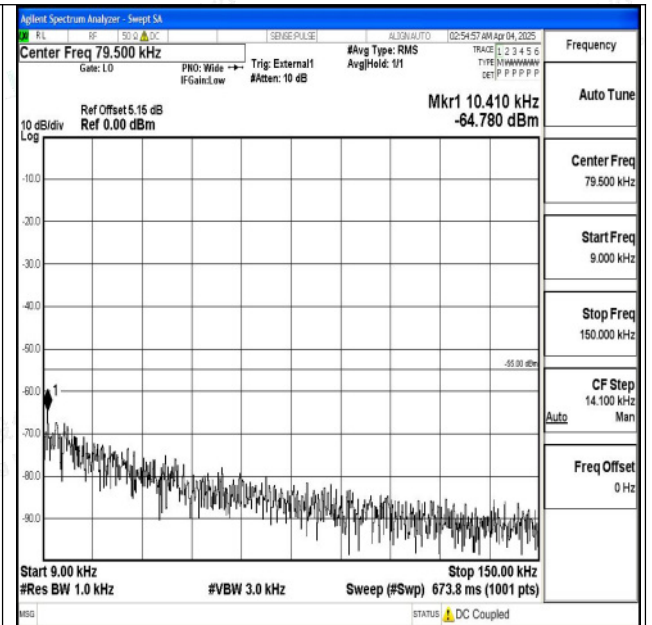
Band38_20MHz_16QAM_38000_1RB#0_0.009~0.15_0. 009~0.15
