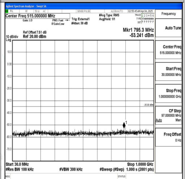
Band38_20MHz_16QAM_38000_1RB#0_30~1000_30~1 000
