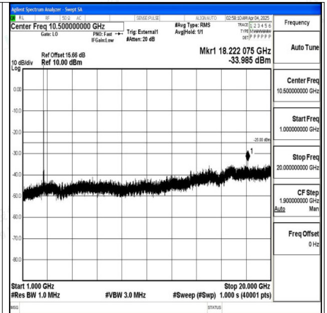
Band38_20MHz_QPSK_38150_1RB#0_1000~20000_1000~20000
