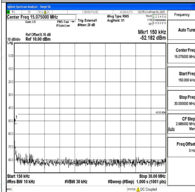
Band38_20MHz_16QAM_38000_1RB#0_0.15~30_0.15~ 30
