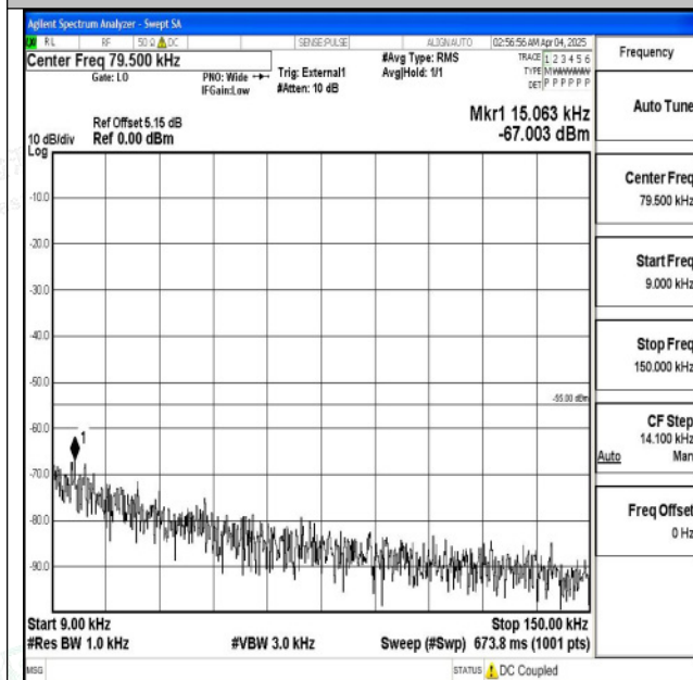
Band38_20MHz_QPSK_38150_1RB#0_0.009~0.15_0.00 9~0.15
