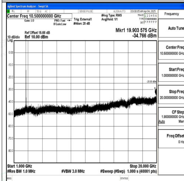
Band38_20MHz_16QAM_38150_1RB#0_1000~20000_1000~20000
