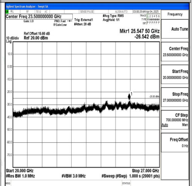
Band38_20MHz_16QAM_38150_1RB#0_20000~27000_20000~27000
