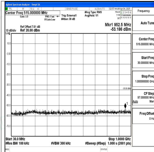
Band38_20MHz_QPSK_38150_1RB#0_30~1000_30~1000
