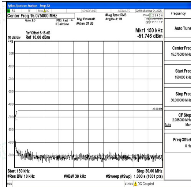
Band38_20MHz_16QAM_38150_1RB#0_0.15~30_0.15~30
