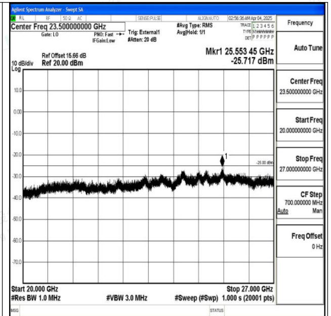
Band38_20MHz_16QAM_38000_1RB#0_20000~27000_2 20000~27000
