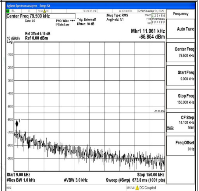
Band38_20MHz_16QAM_38150_1RB#0_0.009~0.15_0.009~0.15
