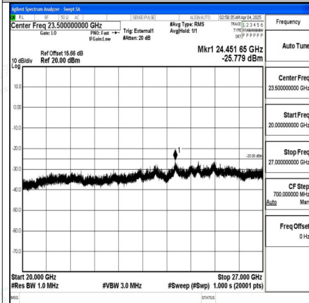
Band38_20MHz_QPSK_38150_1RB#0_20000~27000_20000~27000
