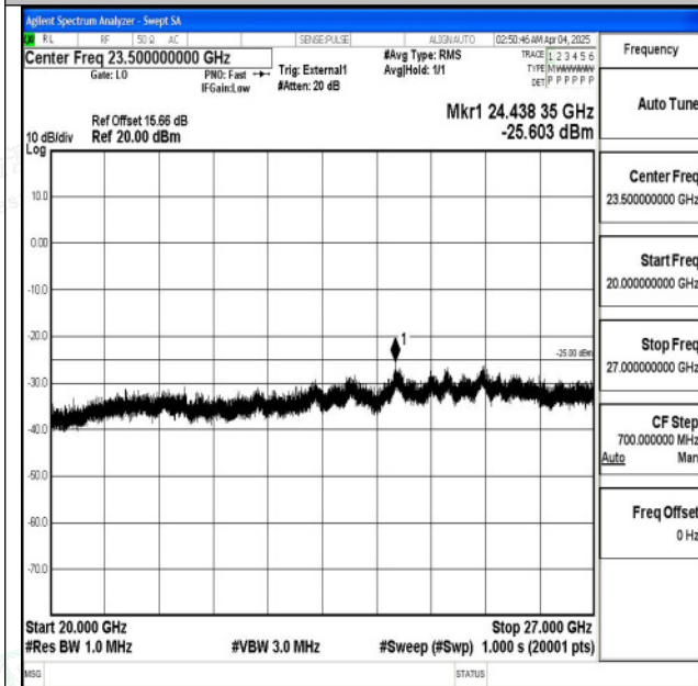
Band38_20MHz_QPSK_37850_1RB#0_20000~27000_20000~27000
