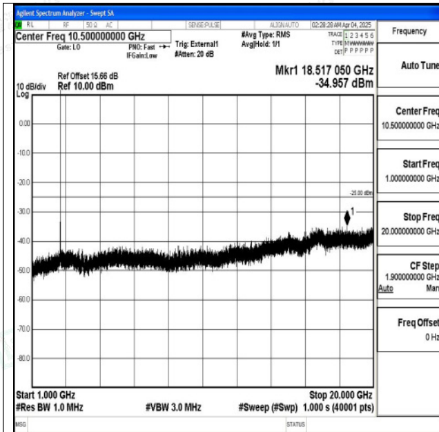
Band38_10MHz_16QAM_38000_1RB#0_1000~20000_1 000~20000
