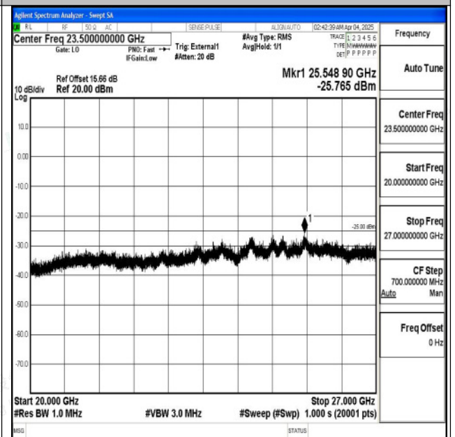
Band38_15MHz_16QAM_38000_1RB#0_20000~27000_20000~27000
