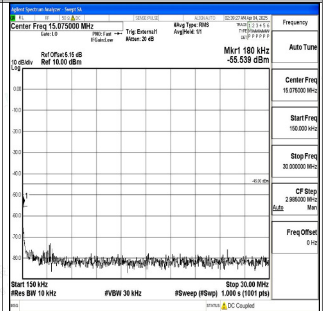
Band38_15MHz_QPSK_38000_1RB#0_0.15~30_0.15~3 0
