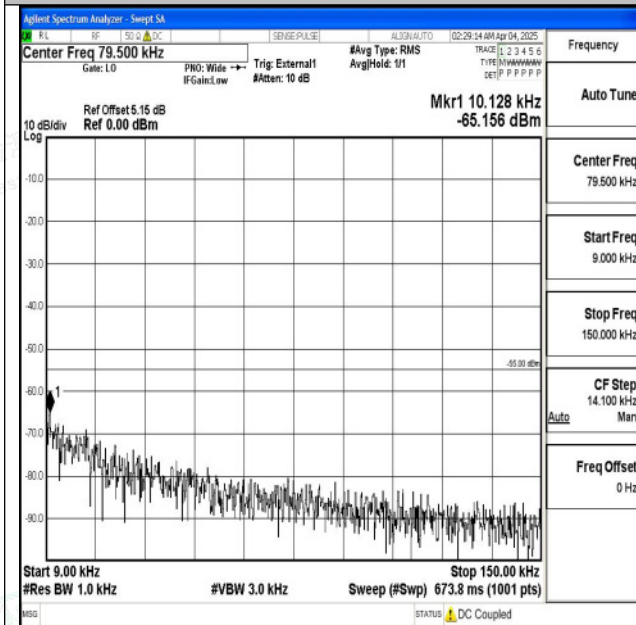
Band38_10MHz_QPSK_38200_1RB#0_0.009~0.15_0.009~0.15 9~0.15
