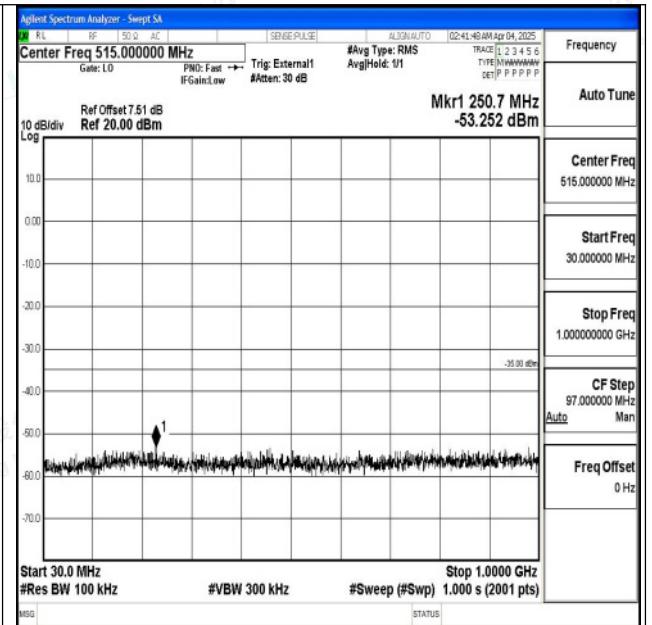
Band38_15MHz_16QAM_38000_1RB#0_30~1000_30~1000
