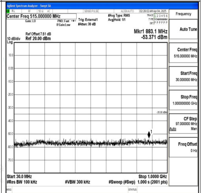
Band38_10MHz_16QAM_38000_1RB#0_30~1000_30~1 000
