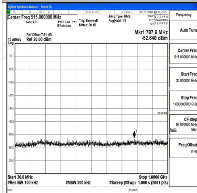
Band38_10MHz_QPSK_38000_1RB#0_30~1000_30~10 00
