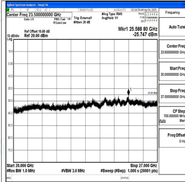
Band38_10MHz_QPSK_38000_1RB#0_20000~27000_2 0000~27000
