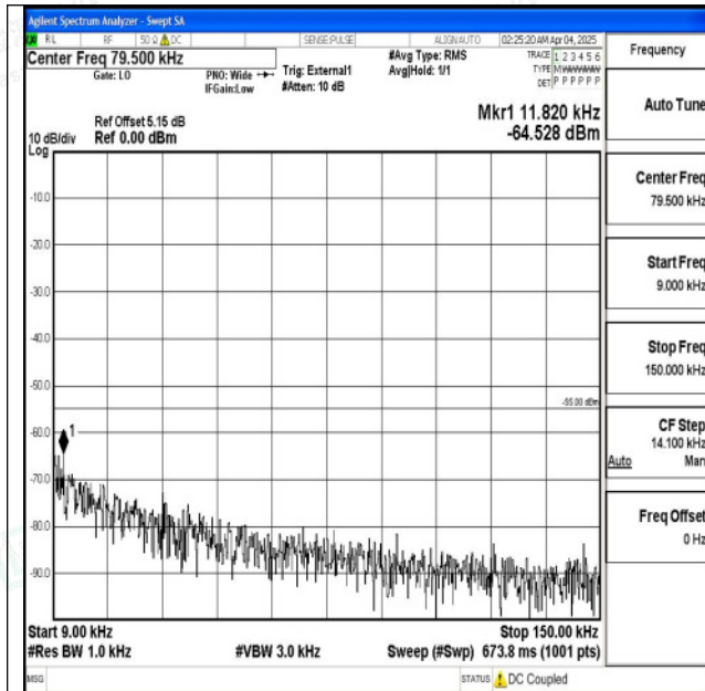
Band38_10MHz_QPSK_38000_1RB#0_0.009~0.15_0.00 9~0.15
