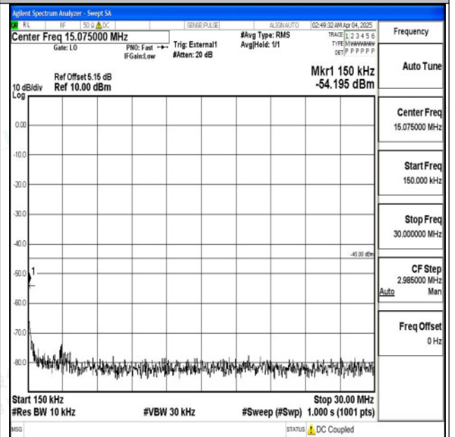
Band38_20MHz_QPSK_37850_1RB#0_0.15~30_0.15~3 0
