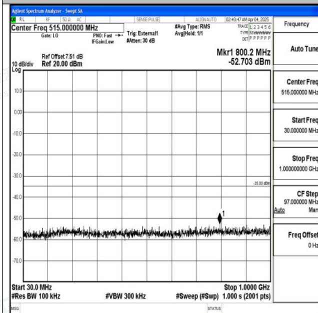
Band38_15MHz_QPSK_38175_1RB#0_30~1000_30~10 00
