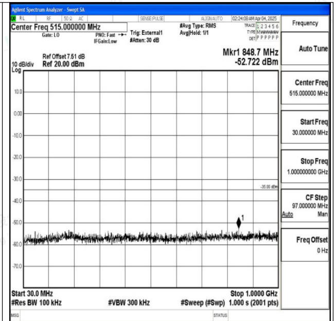
Band38_10MHz_16QAM_37800_1RB#0_30~1000_30~1000
