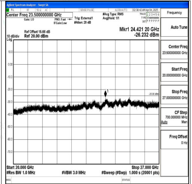
Band38_15MHz_16QAM_37825_1RB#0_20000~27000_ 20000~27000
