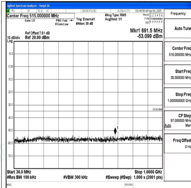
Band38_20MHz_QPSK_37850_1RB#0_30~1000_30~1000
