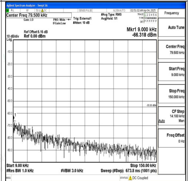
Band38_20MHz_16QAM_37850_1RB#0_0.009~0.15_0.009~0.15
