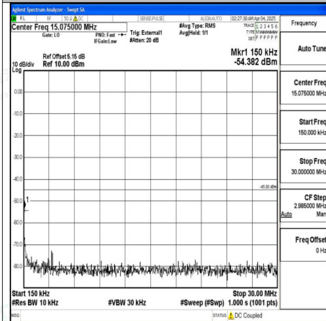
Band38_10MHz_16QAM_38000_1RB#0_0.15~30_0.15~ 30
