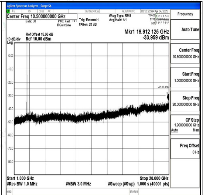
Band38_20MHz_QPSK_37850_1RB#0_1000~20000_1000~20000
