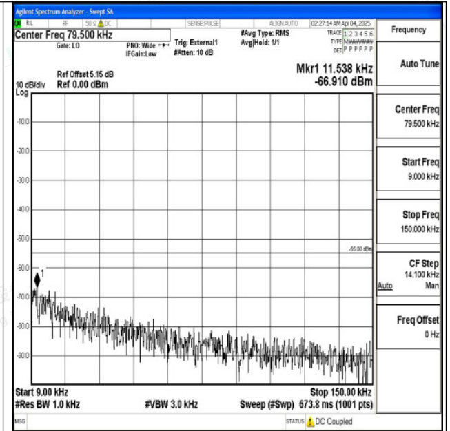
Band38_10MHz_16QAM_38000_1RB#0_0.009~0.15_0. 009~0.15
