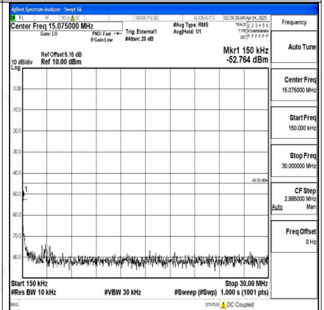
Band38_10MHz_QPSK_38200_1RB#0_0.15~30_0.15~30 0
