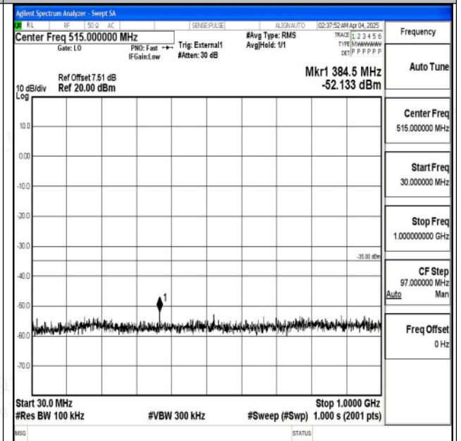
Band38_15MHz_16QAM_37825_1RB#0_30~1000_30~1000 000
