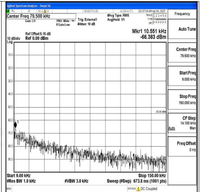
Band38_15MHz_16QAM_37825_1RB#0_0.009~0.15_0. 009~0.15
