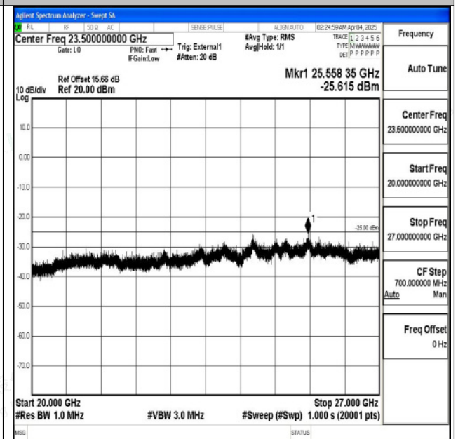
Band38_10MHz_16QAM_37800_1RB#0_20000~27000_20000~27000
