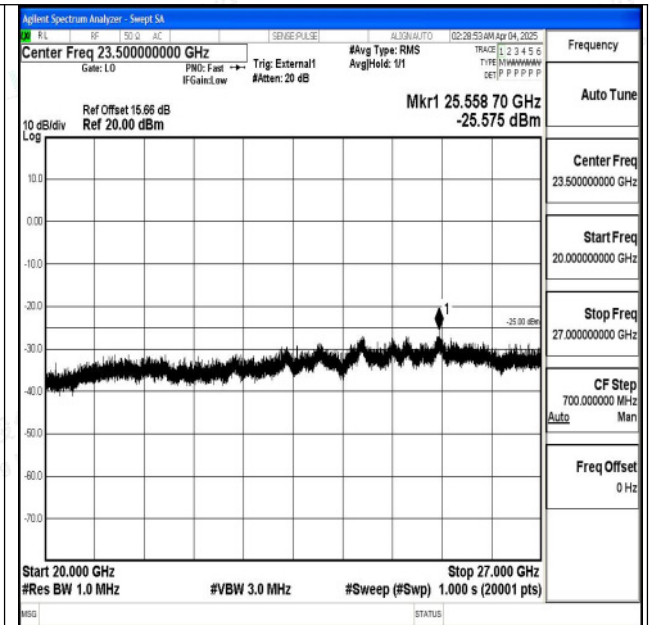
Band38_10MHz_16QAM_38000_1RB#0_20000~27000_2 20000~27000
