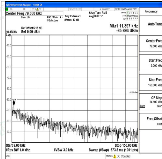
Band38_15MHz_QPSK_38175_1RB#0_0.009~0.15_0.00 9~0.15
