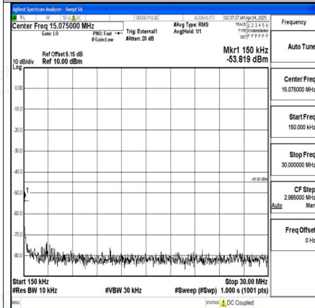
Band38_15MHz_16QAM_37825_1RB#0_0.15~30_0.15~30 30
