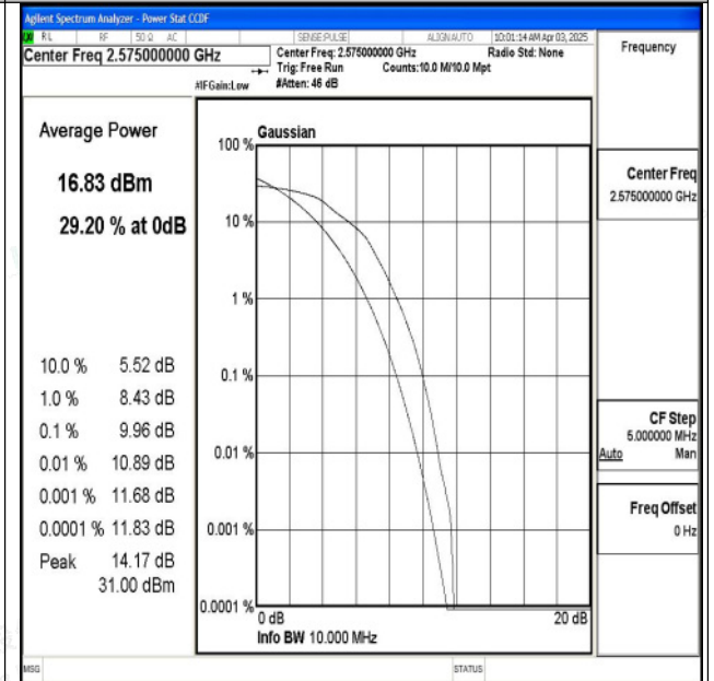
Band38-10MHz-16QAM-37800-50RB#0-PASS
