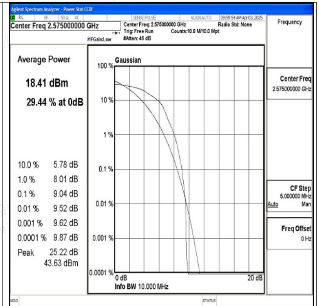
Band38-10MHz-16QAM-37800-1RB#0-PASS
