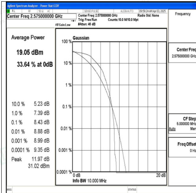
Band38-10MHz-QPSK-37800-1RB#0-PASS
