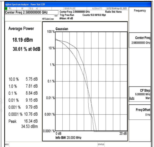
Band38-20MHz-16QAM-37850-1RB#0-PASS
