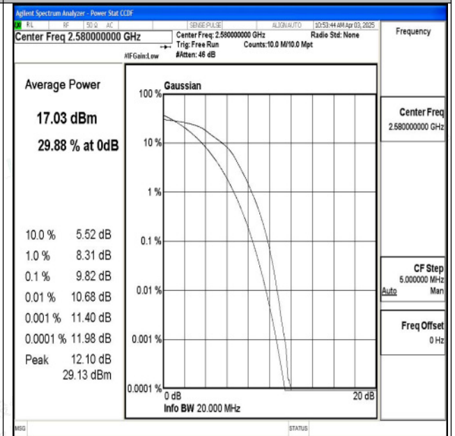
Band38-20MHz-16QAM-37850-100RB#0-PASS
