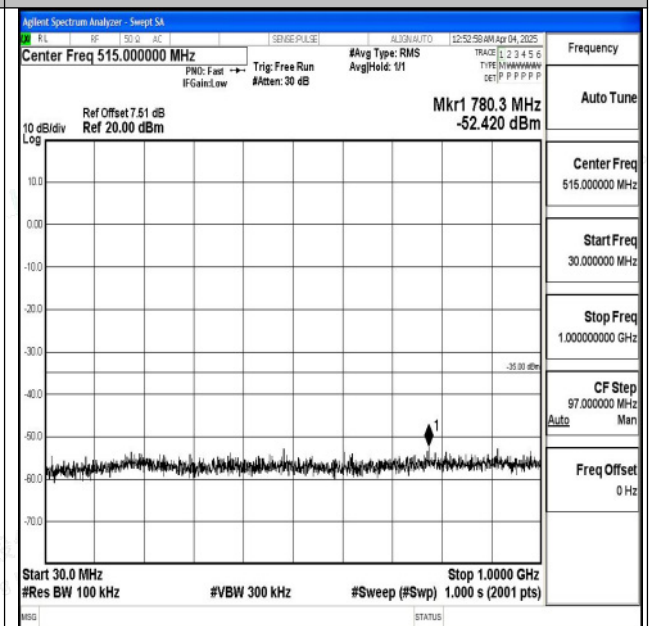
Band7_20MHz_16QAM_21100_1RB#0_30~1000_30~1000
