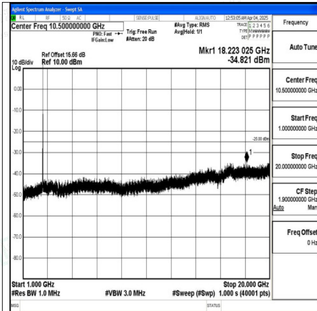
Band7_20MHz_16QAM_21100_1RB#0_1000~20000_1000~20000
