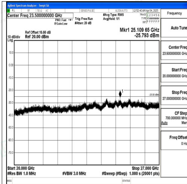
Band7_20MHz_QPSK_21100_1RB#0_20000~27000_2000~27000
