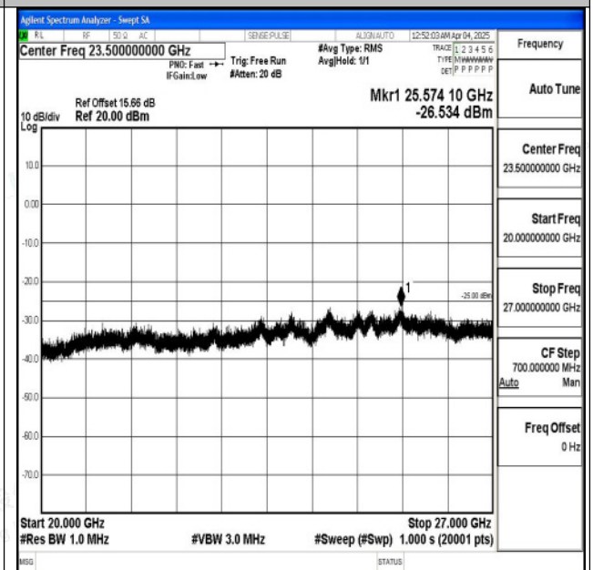
Band7_20MHz_16QAM_20850_1RB#0_20000~27000_2
