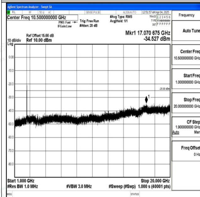
Band7_20MHz_16QAM_20850_1RB#0_1000~20000_10
