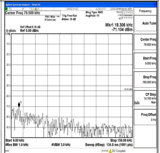
Band7_20MHz_16QAM_20850_1RB#0_0.009~0.15_0.009~0.15 09~0.15
