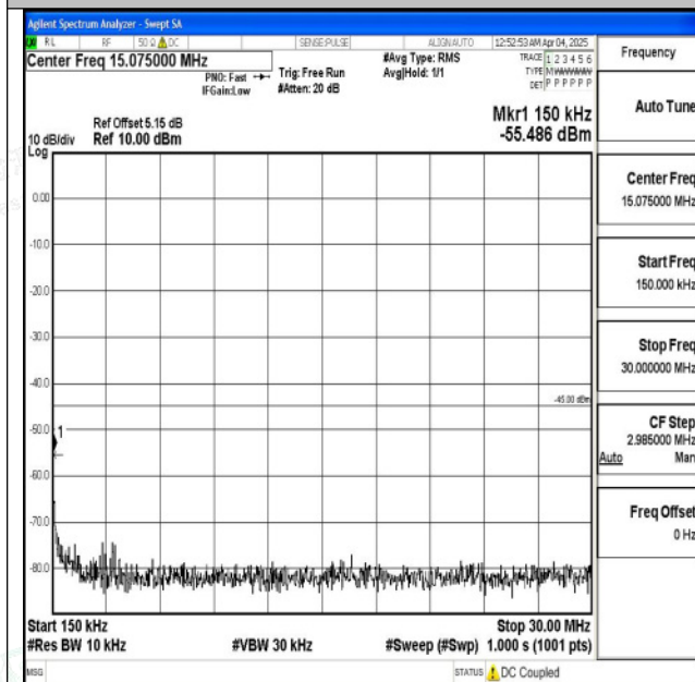
Band7_20MHz_16QAM_21100_1RB#0_0.15~30_0.15~30
