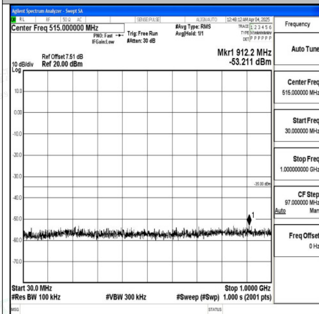
Band7_15MHz_QPSK_21375_1RB#0_30~1000_30~1000
