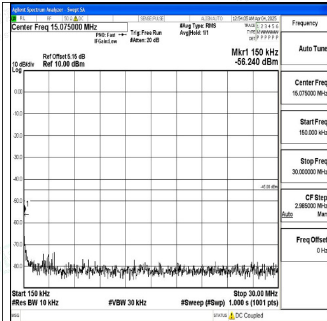
Band7_20MHz_16QAM_21350_1RB#0_0.15~30_0.15~3
