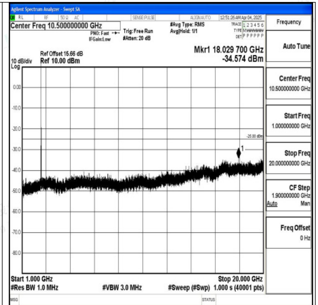
Band7_20MHz_QPSK_20850_1RB#0_1000~20000_1000~20000 0~20000
