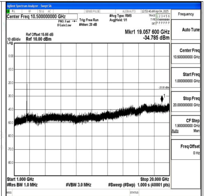
Band7_20MHz_QPSK_21350_1RB#0_1000~20000_1000~20000 0~20000
