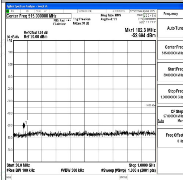
Band7_20MHz_QPSK_21100_1RB#0_30~1000_30~1000
