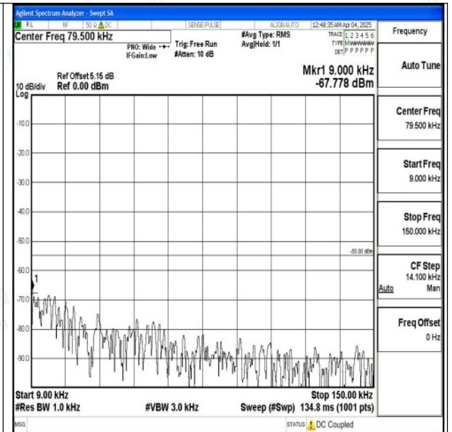
Band7_15MHz_16QAM_21375_1RB#0_0.009~0.15_0.009~0.15
