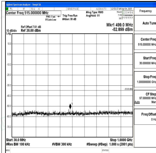
Band7_20MHz_QPSK_21350_1RB#0_30~1000_30~1000 0
