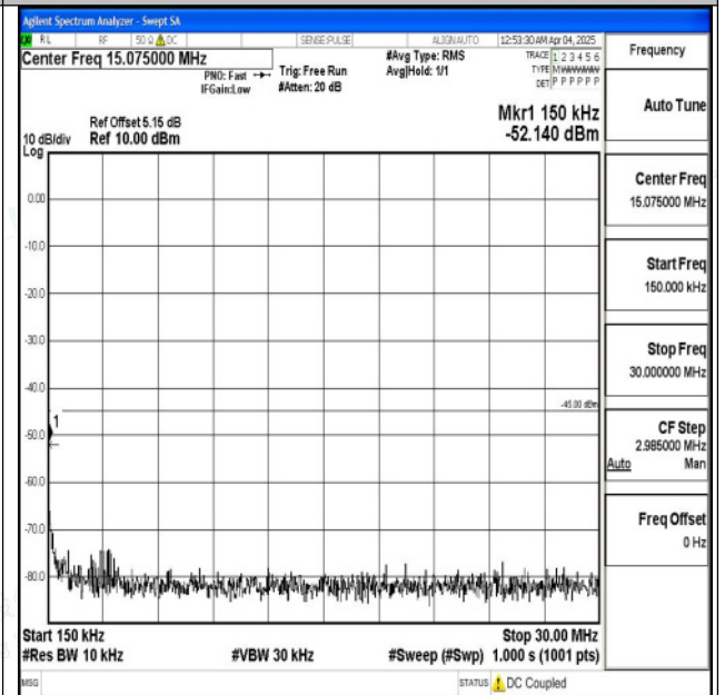
Band7_20MHz_QPSK_21350_1RB#0_0.15~30_0.15~30
