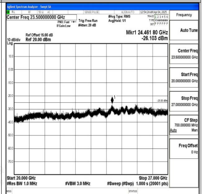
Band7_20MHz_16QAM_21350_1RB#0_20000~27000_2
