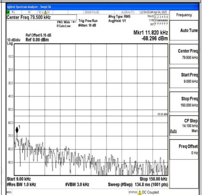
Band7_20MHz_16QAM_21350_1RB#0_0.009~0.15_0.009~0.15 09~0.15
