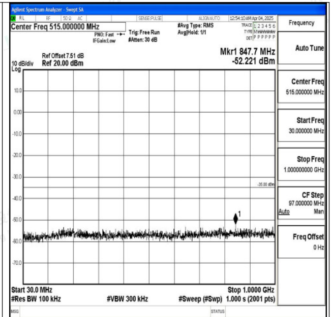
Band7_20MHz_16QAM_21350_1RB#0_30~1000_30~10
