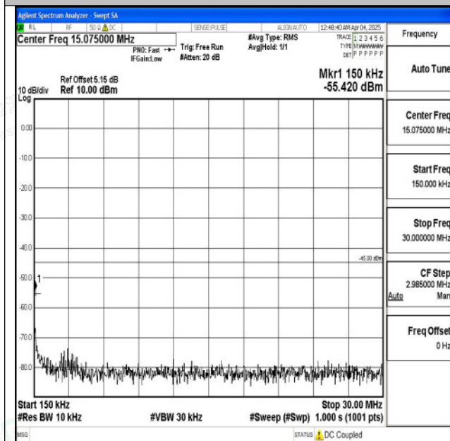
Band7_15MHz_16QAM_21375_1RB#0_0.15~30_0.15~30
