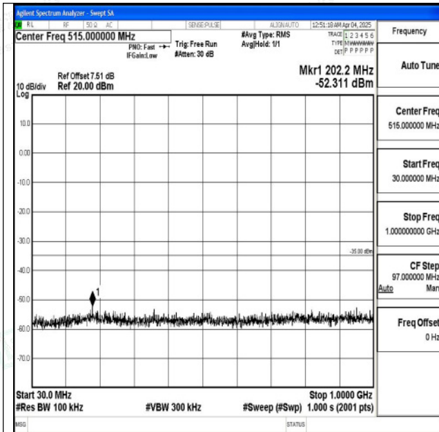
Band7_20MHz_QPSK_20850_1RB#0_30~1000_30~1000 0
