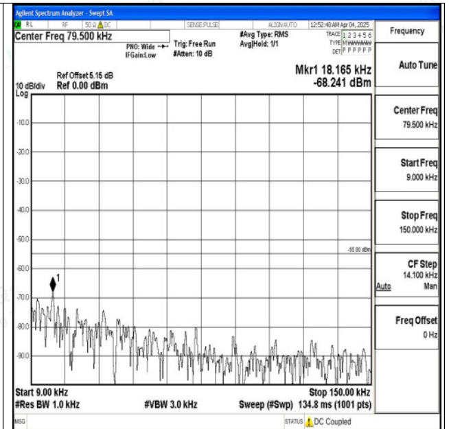
Band7_20MHz_16QAM_21100_1RB#0_0.009~0.15_0.009~0.15
