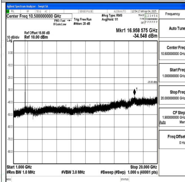
Band7_20MHz_16QAM_21350_1RB#0_1000~20000_10
