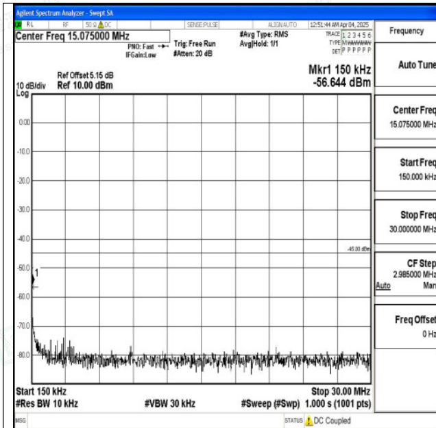
Band7_20MHz_16QAM_20850_1RB#0_0.15~30_0.15~3
