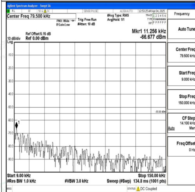
Band7_20MHz_QPSK_21350_1RB#0_0.009~0.15_0.009~0.15
