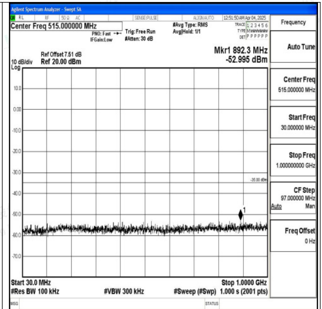
Band7_20MHz_16QAM_20850_1RB#0_30~1000_30~10
