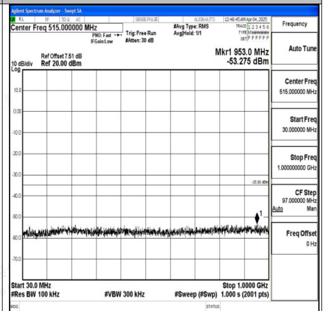
Band7_15MHz_16QAM_21375_1RB#0_30~1000_30~1000
