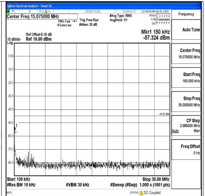
Band7_15MHz_QPSK_21375_1RB#0_0.15~30_0.15~30
