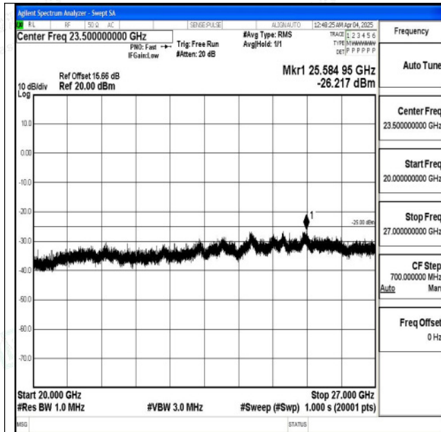
Band7_15MHz_QPSK_21375_1RB#0_20000~27000_2000~27000
