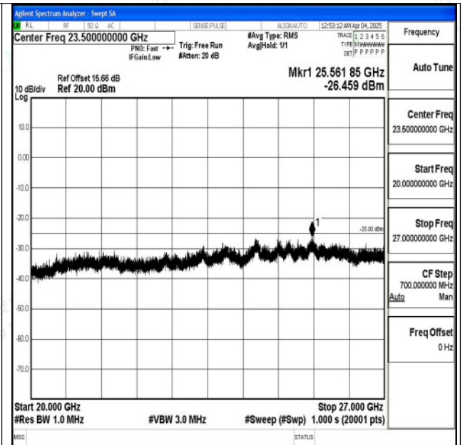
Band7_20MHz_16QAM_21100_1RB#0_20000~27000_20000~27000
